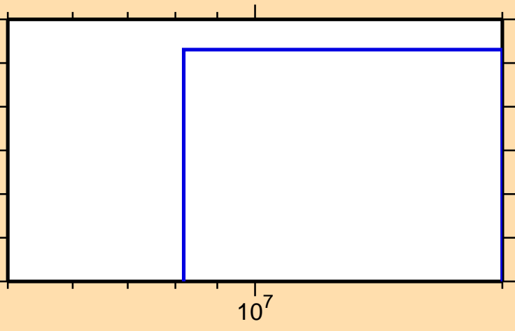
\sigma vs. E for ^{77}\text{Zn}(n,np)
