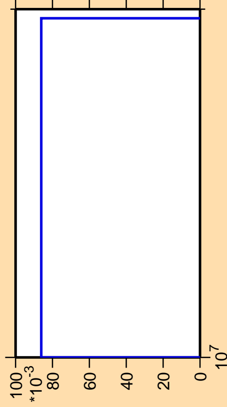
\Delta\sigma/\sigma vs. E for ^{78}\text{Zn}(n,nt)
