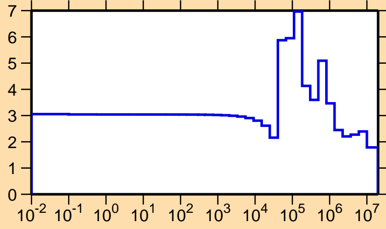
\sigma vs. E for ^{78}\text{Zn}(n,\text{el.})
