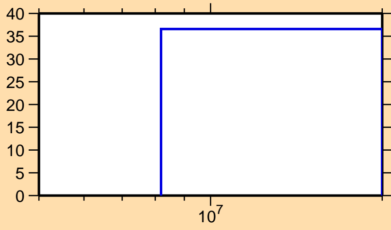
\Delta\sigma/\sigma vs. E for ^{78}\text{Zn}(n,n_1)
