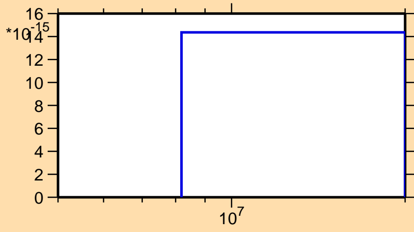
\sigma vs. E for ^{78}\text{Zn}(n,nt)
