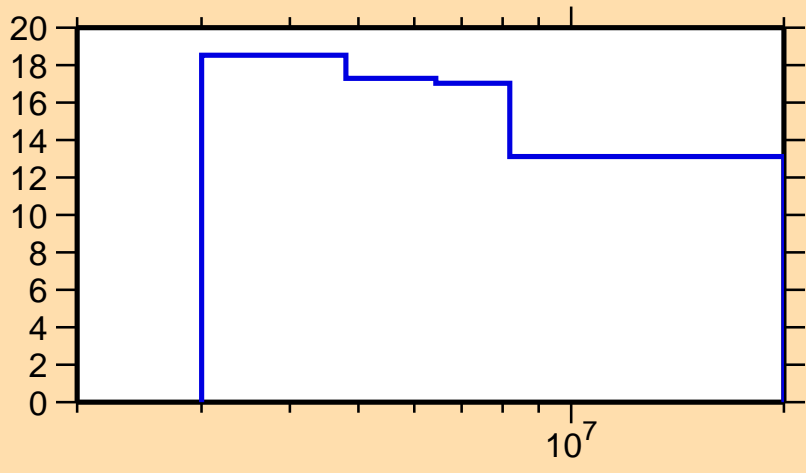
\Delta\sigma/\sigma vs. E for ^{78}\text{Zn}(n,n\text{onel.})
