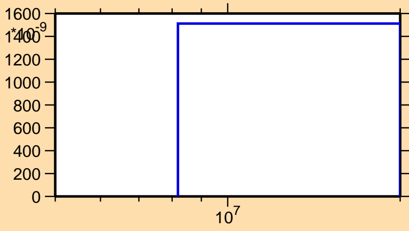
\sigma vs. E for ^{78}\text{Zn}(n,p)
