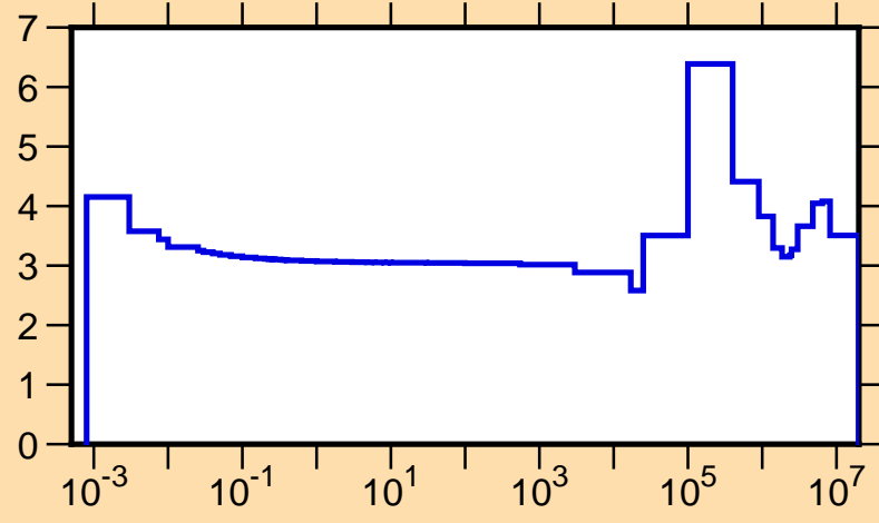
\sigma vs. E for ^{78}\text{Zn}(n,\text{tot.})
