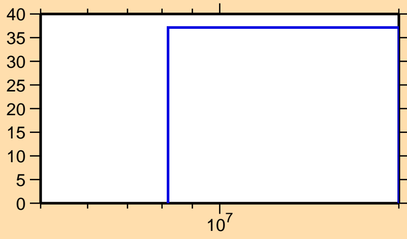
\Delta\sigma/\sigma vs. E for ^{78}\text{Zn}(n,ncont.)
