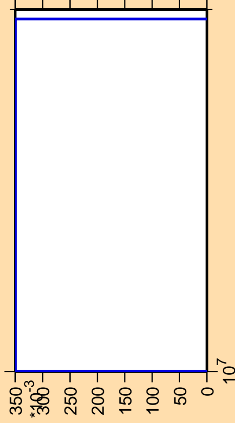
\Delta\sigma/\sigma vs. E for ^{80}\text{Zr}(n,nd)
