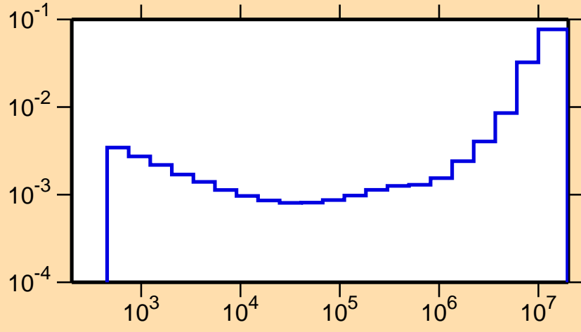
\sigma vs. E for ^{80}\text{Zr}(n,\alpha)
