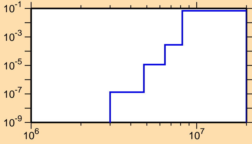
\sigma vs. E for ^{80}\text{Zr}(n,p\alpha)
