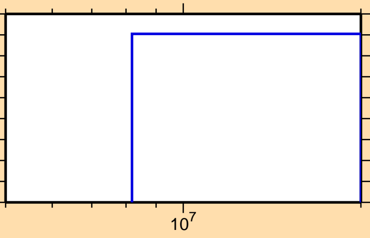
\sigma vs. E for ^{80}\text{Zr}(n,2n)
