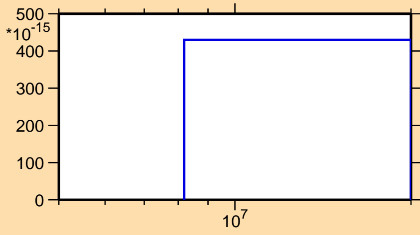
\sigma vs. E for ^{80}\text{Zr} (mt 34)
