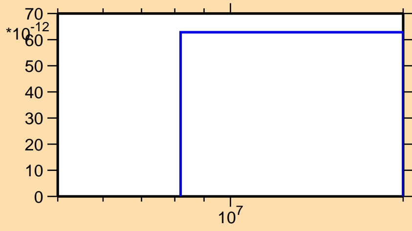
\sigma vs. E for ^{80}\text{Zr}(\text{mt } 45)
