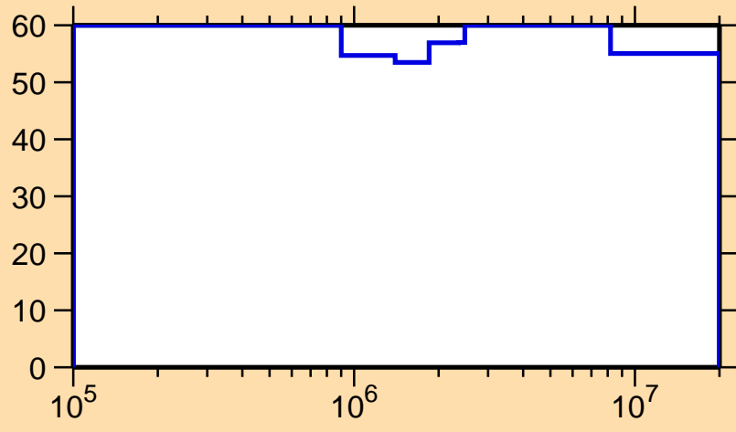
\Delta\sigma/\sigma vs. E for ^{80}\text{Zr}(n,\text{inel.})
