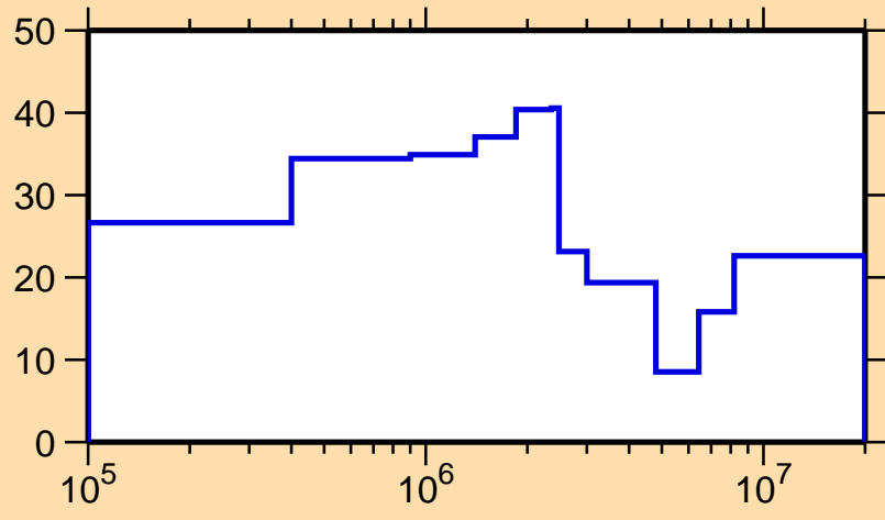
\Delta\sigma/\sigma vs. E for ^{80}\text{Zr}(n,\text{el.})
