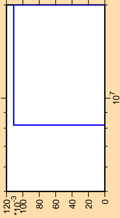
\Delta\sigma/\sigma vs. E for ^{80}\text{Zr}(n,2np)
