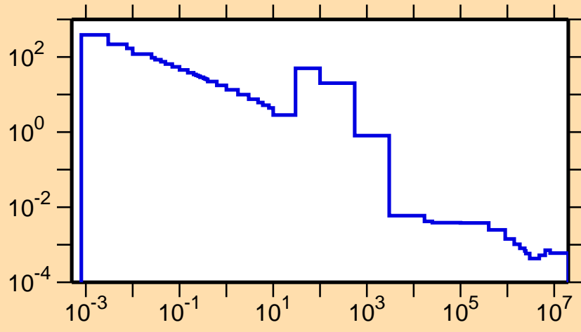
\sigma vs. E for ^{80}\text{Zr}(n,\gamma)
