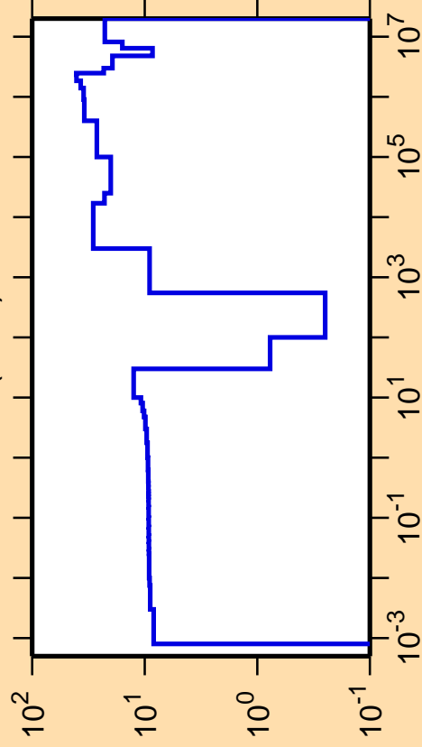
\Delta\sigma/\sigma vs. E for ^{80}\text{Zr}(n,\text{el.})
