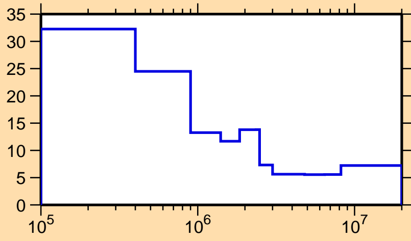
\Delta\sigma/\sigma vs. E for ^{80}\text{Zr}(n,\text{nonel.})
