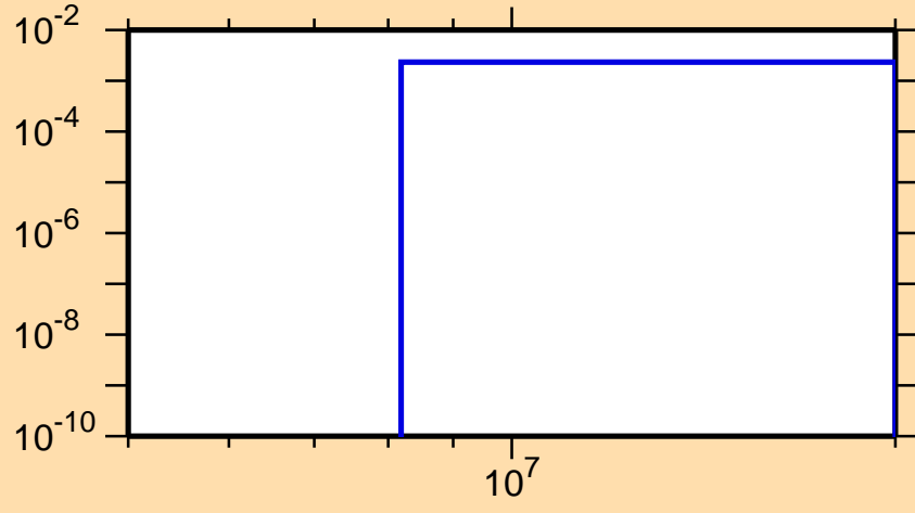
\sigma vs. E for ^{80}\text{Zr}(n,\text{pd})
