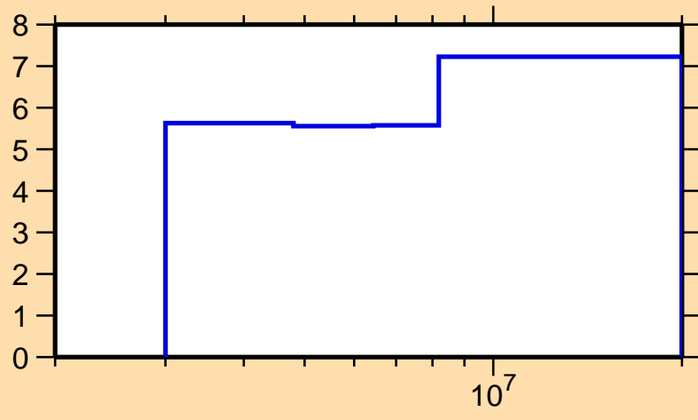
\Delta\sigma/\sigma vs. E for ^{80}\text{Zr}(n,n\text{onel.})
