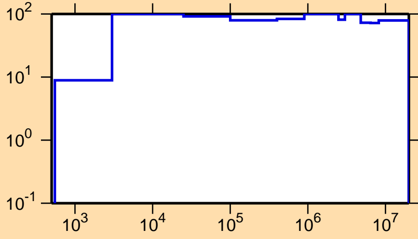
\Delta\sigma/\sigma vs. E for ^{80}\text{Zr}(n,\gamma)
