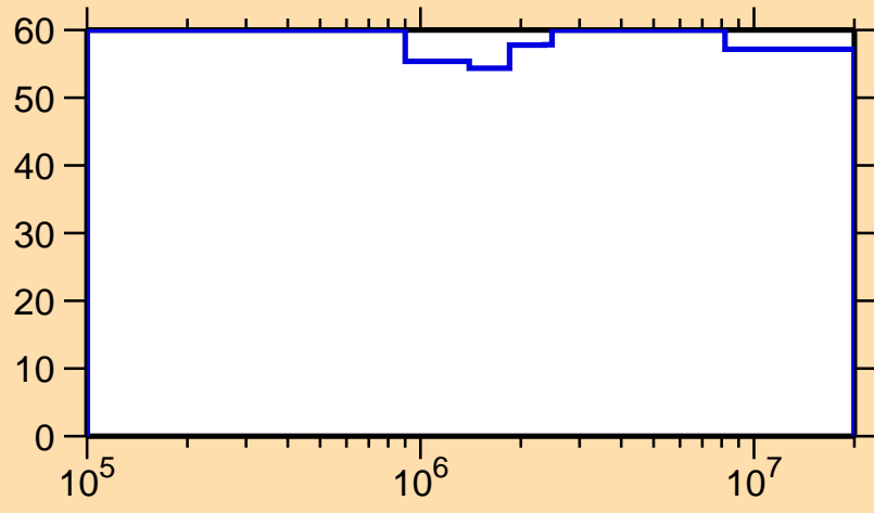
\Delta\sigma/\sigma vs. E for ^{80}\text{Zr}(n,n_1)
