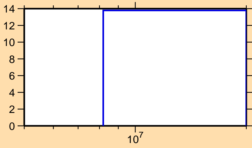
\Delta\sigma/\sigma vs. E for ^{80}\text{Zr}(n,\text{tot.})
