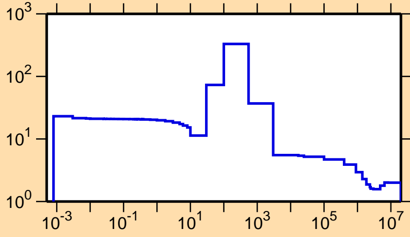
\sigma vs. E for ^{80}\text{Zr}(n,\text{el.})
