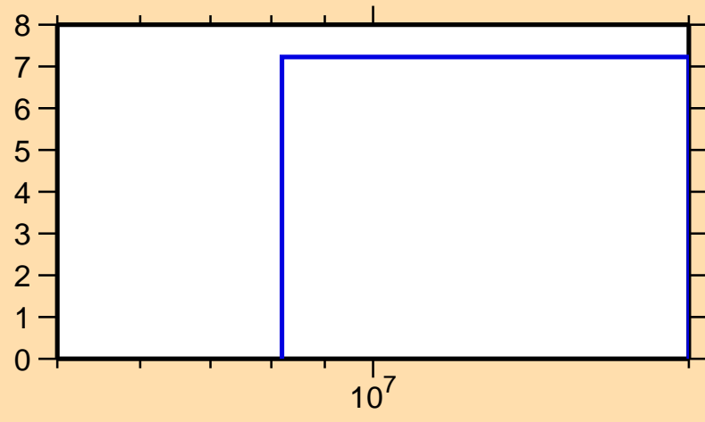
\Delta\sigma/\sigma vs. E for ^{80}\text{Zr}(n,\text{nonel.})
