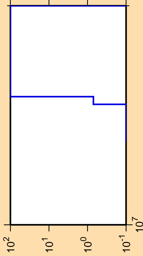
\Delta\sigma/\sigma vs. E for ^{81}\text{Zr}(n,nd)
