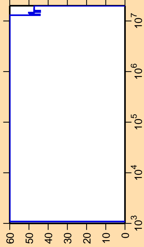
\Delta\sigma/\sigma vs. E for ^{81}\text{Zr}(n,\alpha)
