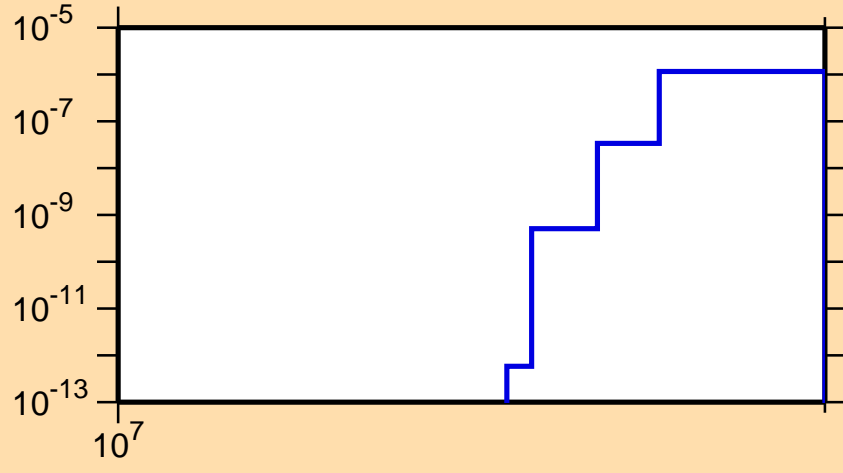
\sigma vs. E for ^{81}\text{Zr}(n,nd)
