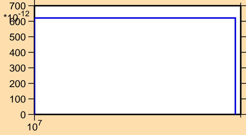
\sigma vs. E for ^{81}\text{Zr} (mt 34)
