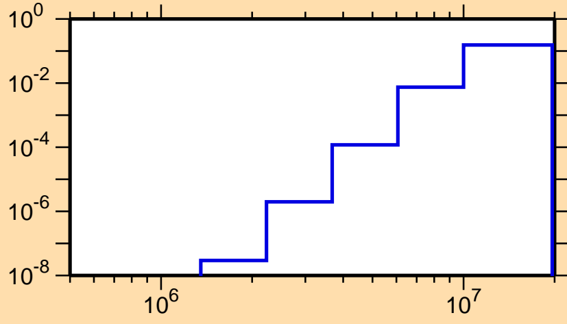
\sigma vs. E for ^{81}\text{Zr}(n,p\alpha)
