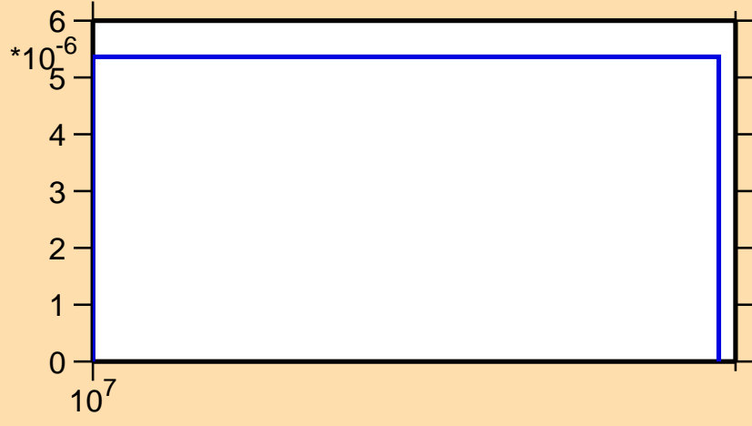
\sigma vs. E for ^{81}\text{Zr}(n,\text{pt})
