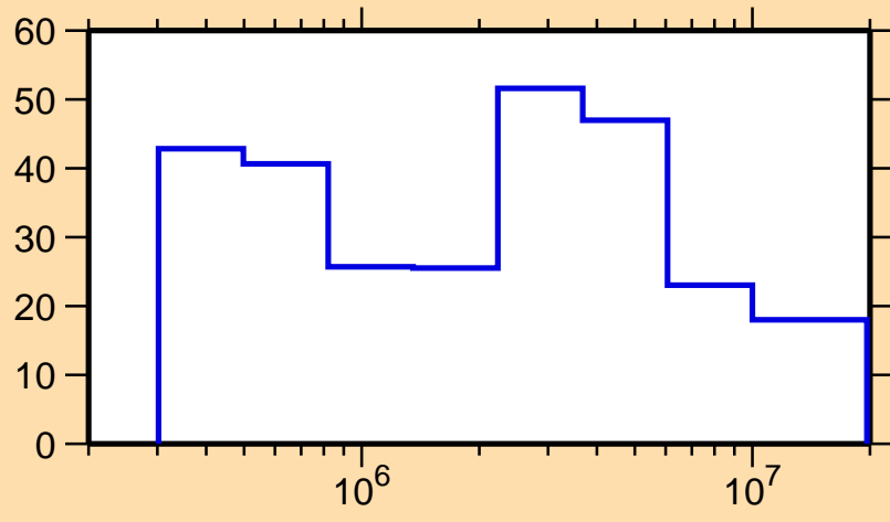
\Delta\sigma/\sigma vs. E for ^{81}\text{Zr}(n, el.)
