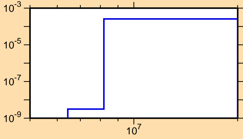
\sigma vs. E for ^{81}\text{Zr}(n,n\alpha)
