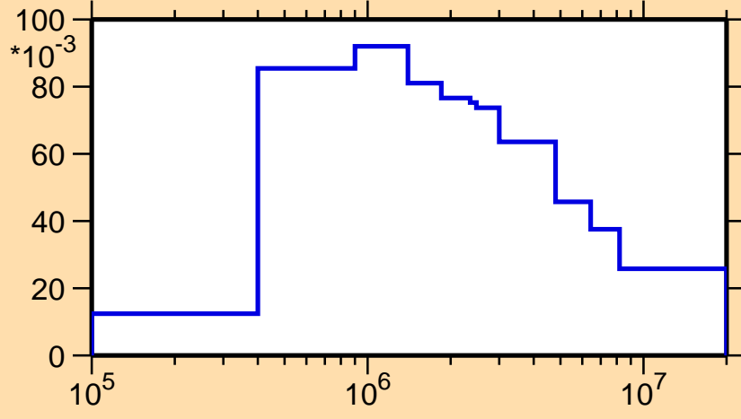
\sigma vs. E for ^{81}\text{Zr}(n,n_3)
