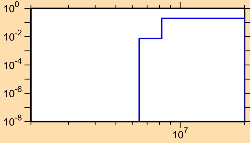
\sigma vs. E for ^{81}\text{Zr}(n,np)
