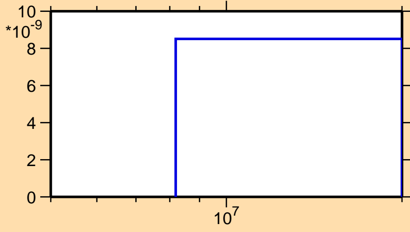
\sigma vs. E for ^{81}\text{Zr}(\text{mt } 45)
