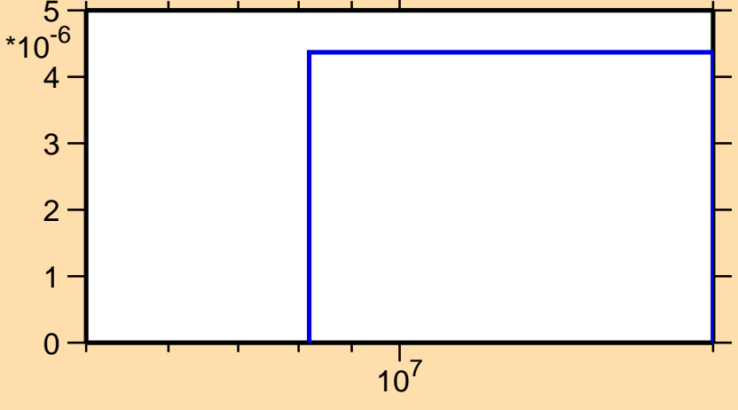
\sigma vs. E for ^{81}\text{Zr}(n,\text{pt})
