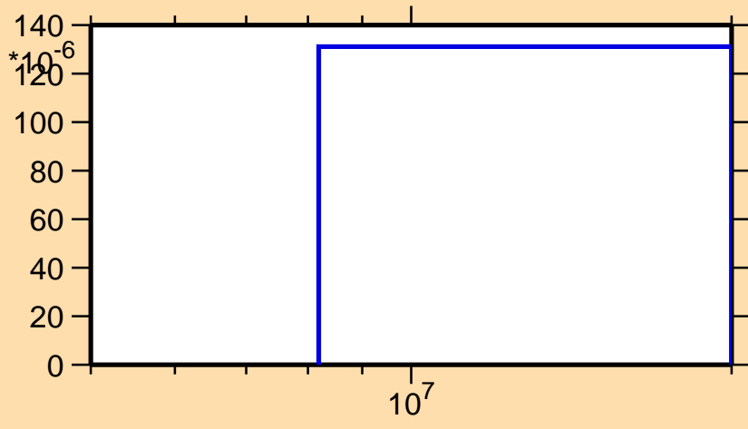
\sigma vs. E for ^{81}\text{Zr}(n,t)
