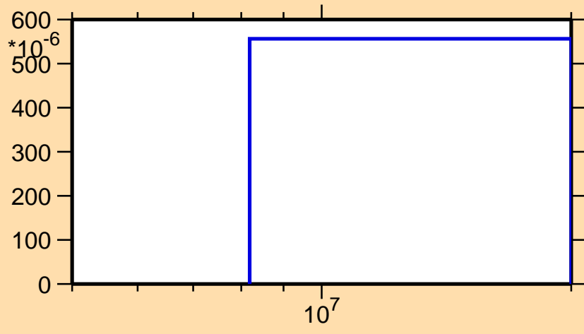
\sigma vs. E for ^{81}\text{Zr}(n,2n)
