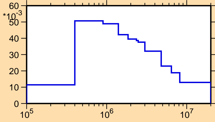
\sigma vs. E for ^{81}\text{Zr}(n,n_1)
