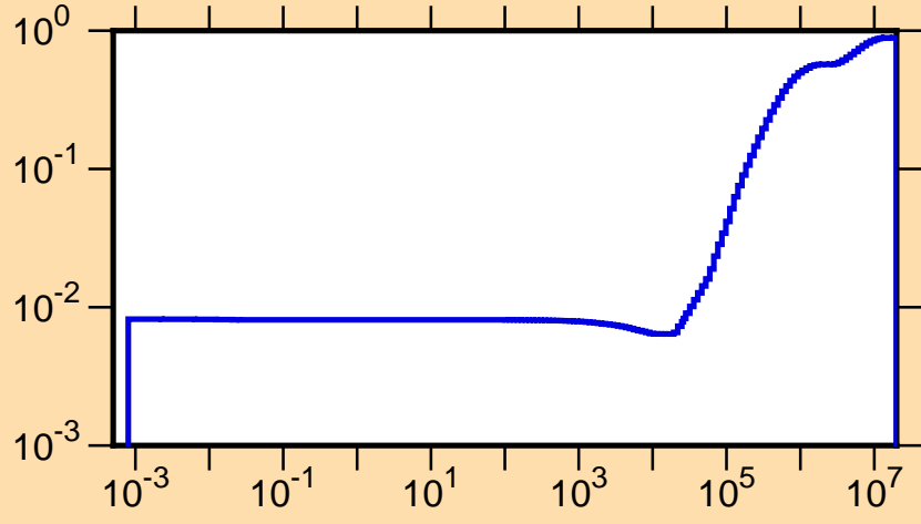
\mu vs. E for ^{82}\text{Zr}(\text{mt251})
