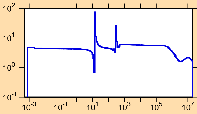
\sigma vs. E for ^{82}\text{Zr}(n,\text{el.})
