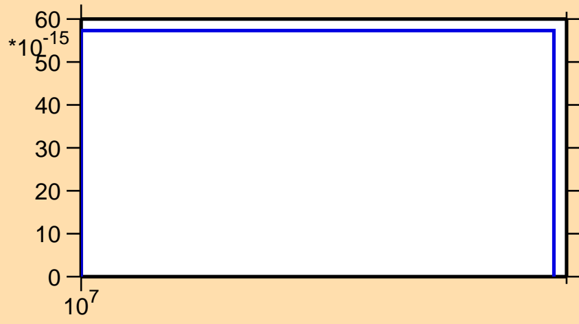
\sigma vs. E for ^{82}\text{Zr} (mt 34)
