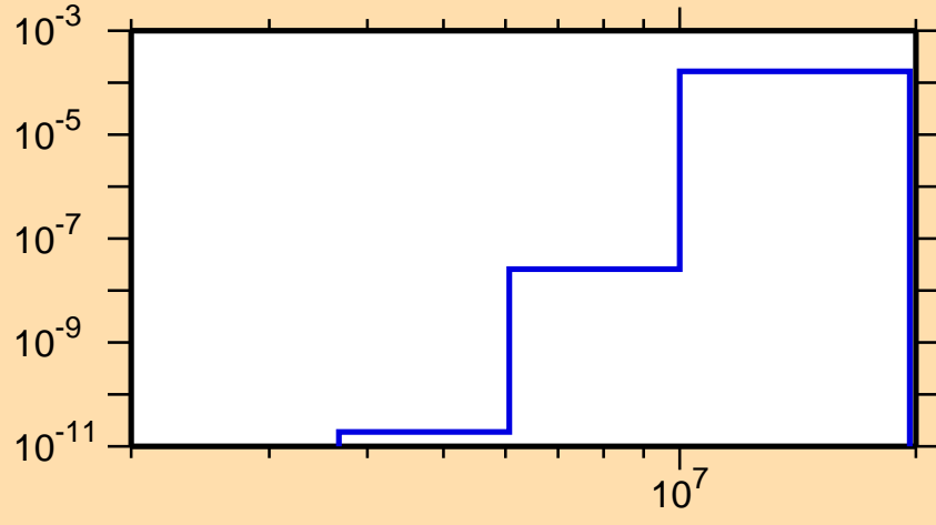
\sigma vs. E for ^{82}\text{Zr}(n,\text{He3})
