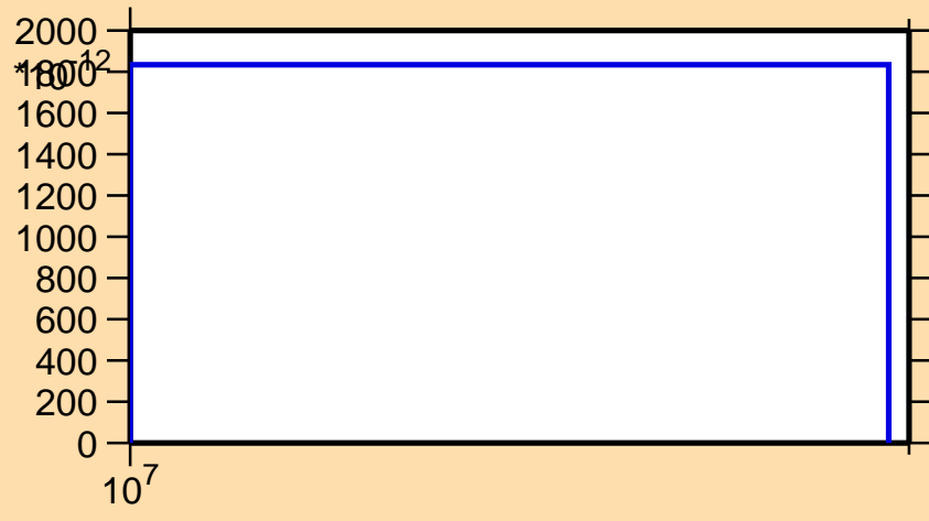
\sigma vs. E for ^{82}\text{Zr} (mt 45)
