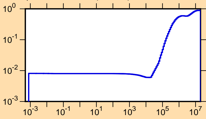
\mu vs. E for ^{83}\text{Zr}(\text{mt251})
