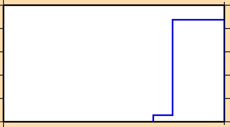
\sigma vs. E for ^{83}\text{Zr}(n,2n\alpha)
