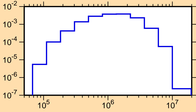
\sigma vs. E for ^{83}\text{Zr}(n,n_2)
