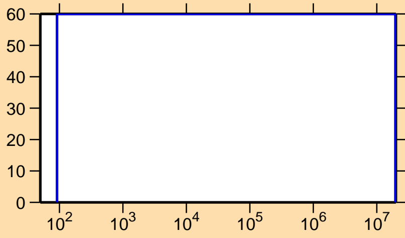
\Delta\sigma/\sigma vs. E for ^{83}\text{Zr}(n,\gamma)
