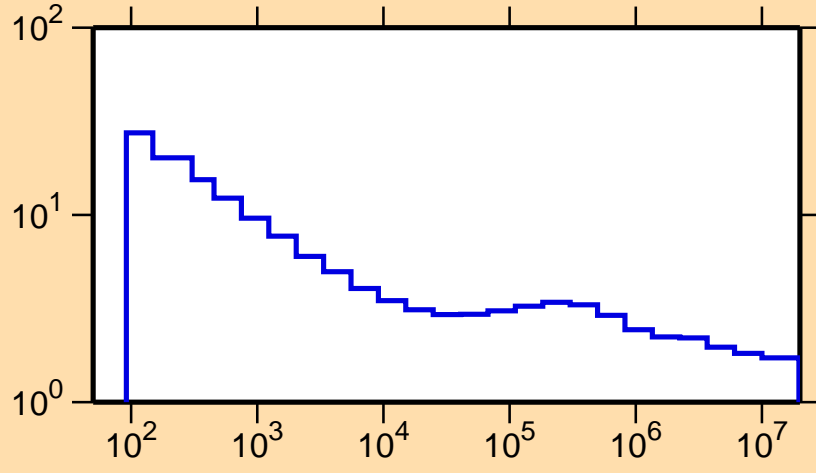
\sigma vs. E for ^{83}\text{Zr}(n,\text{nonel.})
