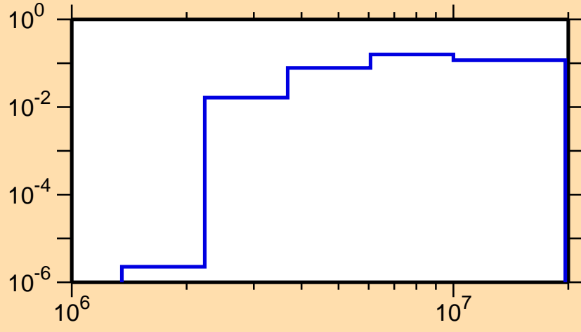
\sigma vs. E for ^{83}\text{Zr}(n,n\text{cont.})
