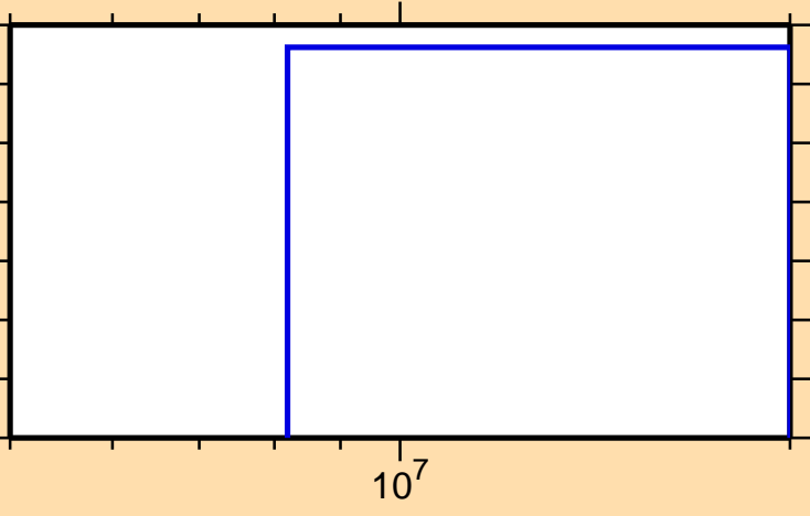
\sigma vs. E for ^{83}\text{Zr}(\text{mt } 45)
