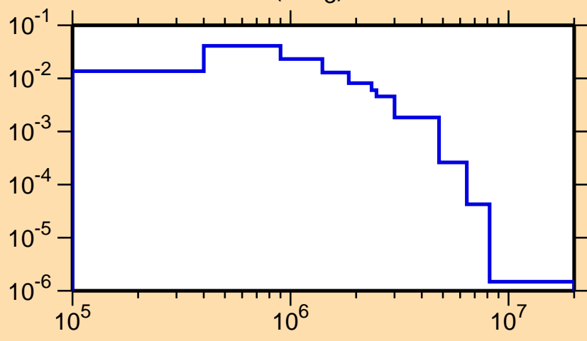
\sigma vs. E for ^{83}\text{Zr}(n,n_3)
