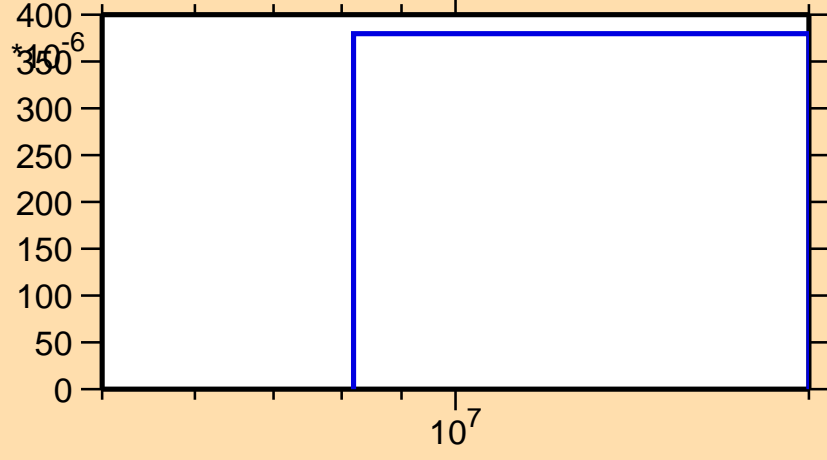
\sigma vs. E for ^{83}\text{Zr}(n,\text{pd})
