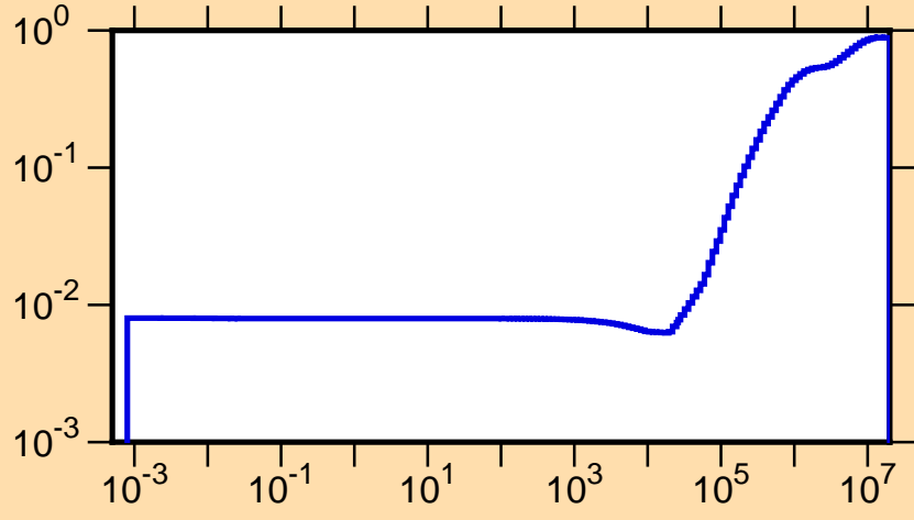
\mu vs. E for ^{84}\text{Zr}(\text{mt251})
