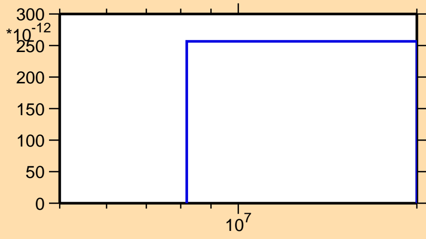
\sigma vs. E for ^{84}\text{Zr}(\text{mt } 45)
