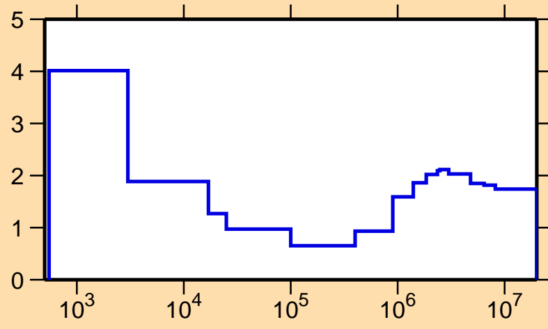
\sigma vs. E for ^{84}\text{Zr}(n,\text{nonel.})
