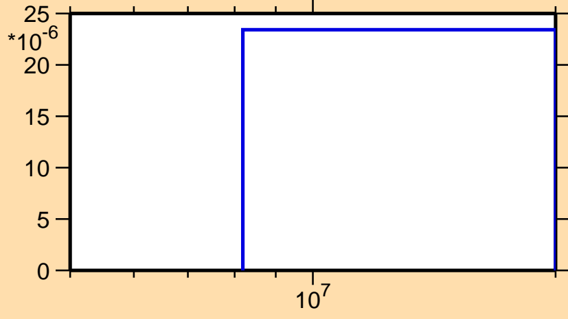
\sigma vs. E for ^{84}\text{Zr}(n,\text{pd})
