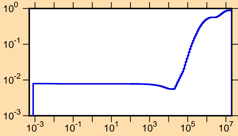
\mu vs. E for ^{85}\text{Zr}(\text{mt251})
