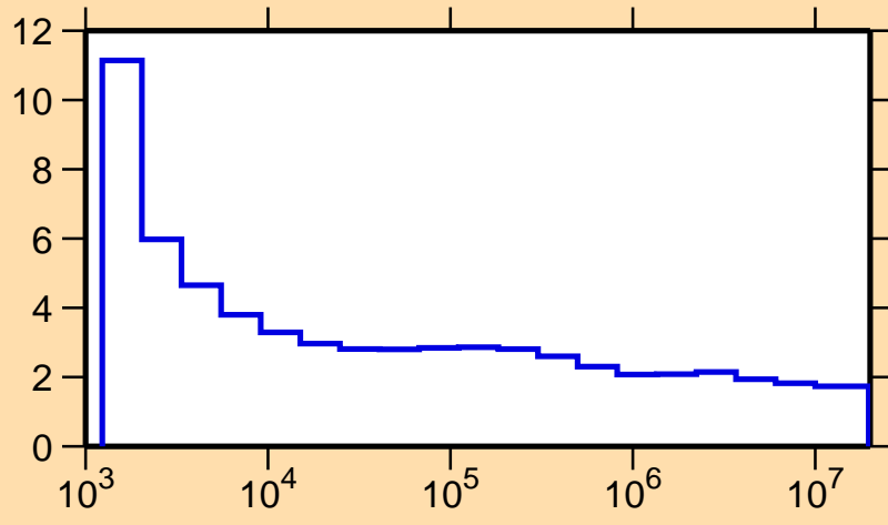
\sigma vs. E for ^{85}\text{Zr}(n,\text{nonel.})
