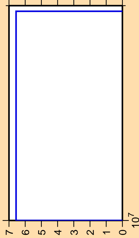
\Delta\sigma/\sigma vs. E for ^{85}\text{Zr} (mt 45)
