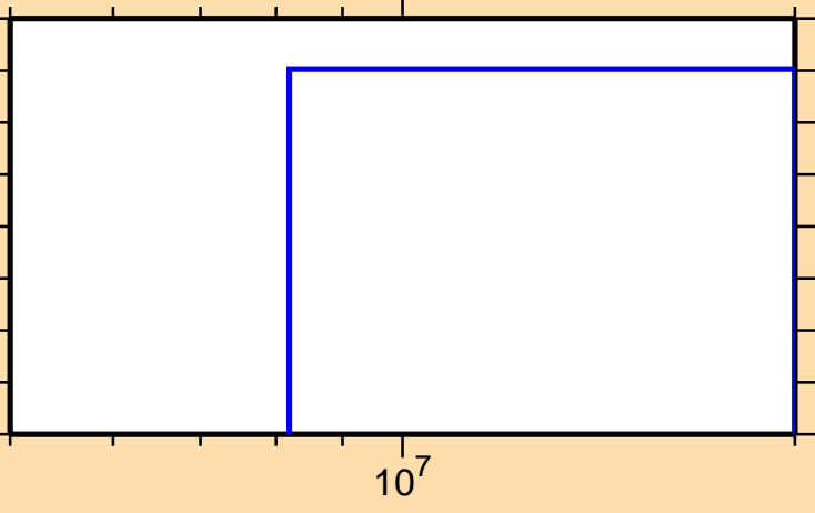
\sigma vs. E for ^{85}\text{Zr}(n,2n\alpha)
