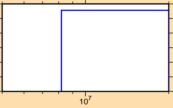
\sigma vs. E for ^{85}\text{Zr}(n,\text{pt})
