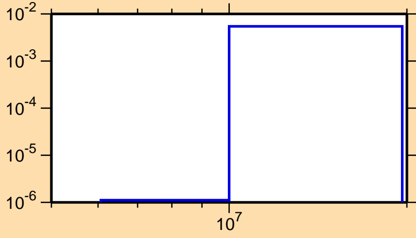
\sigma vs. E for ^{85}\text{Zr}(n,n\alpha)
