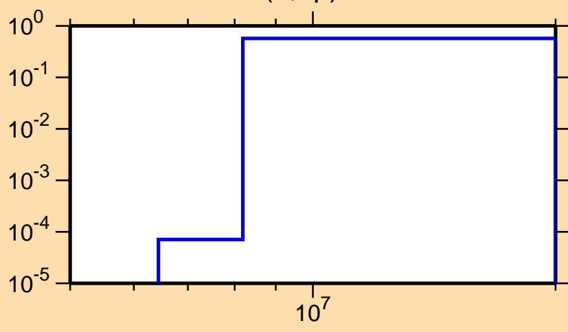
\sigma vs. E for ^{85}\text{Zr}(n,np)
