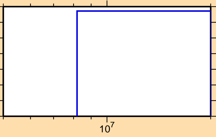
\sigma vs. E for ^{85}\text{Zr}(n,\text{nd})
