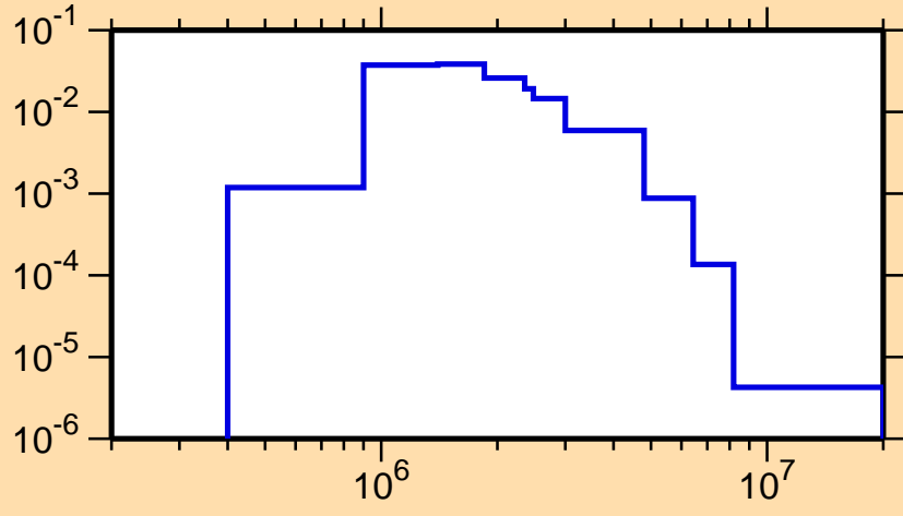
\sigma vs. E for ^{85}\text{Zr}(n,n_4)
