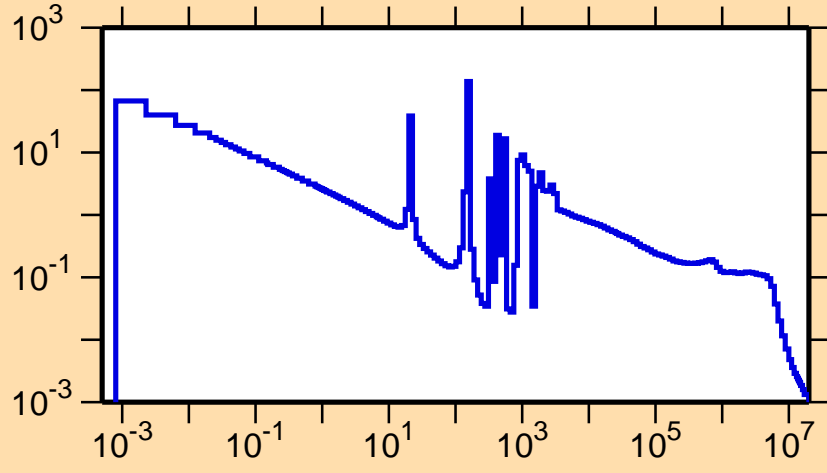
\sigma vs. E for ^{86}\text{Zr}(n,\gamma)
