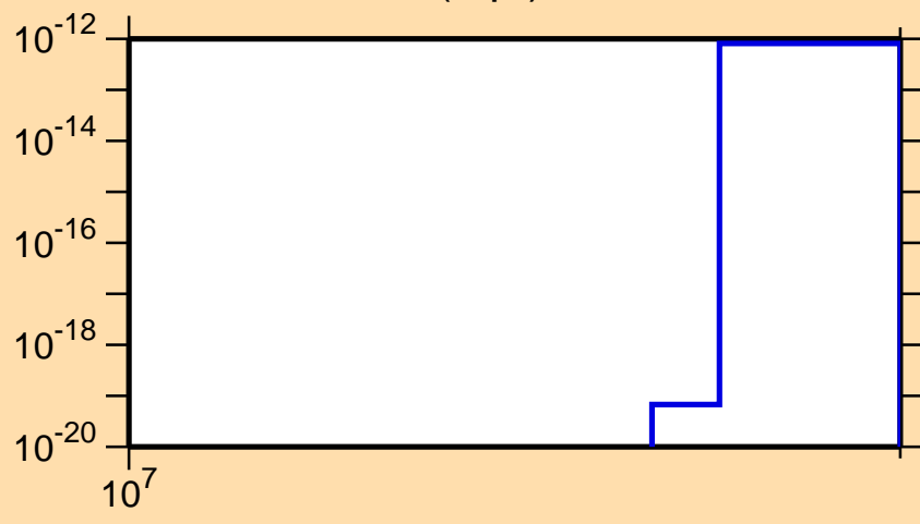
\sigma vs. E for ^{86}\text{Zr}(n,\text{pt})
