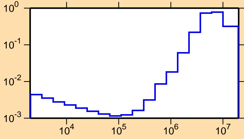
\sigma vs. E for ^{86}\text{Zr}(n,p)
