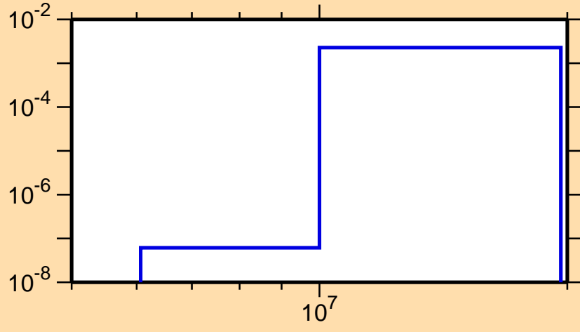
\sigma vs. E for ^{86}\text{Zr}(n,n\alpha)
