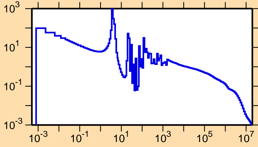
\sigma vs. E for ^{87}\text{Zr}(n,\gamma)
