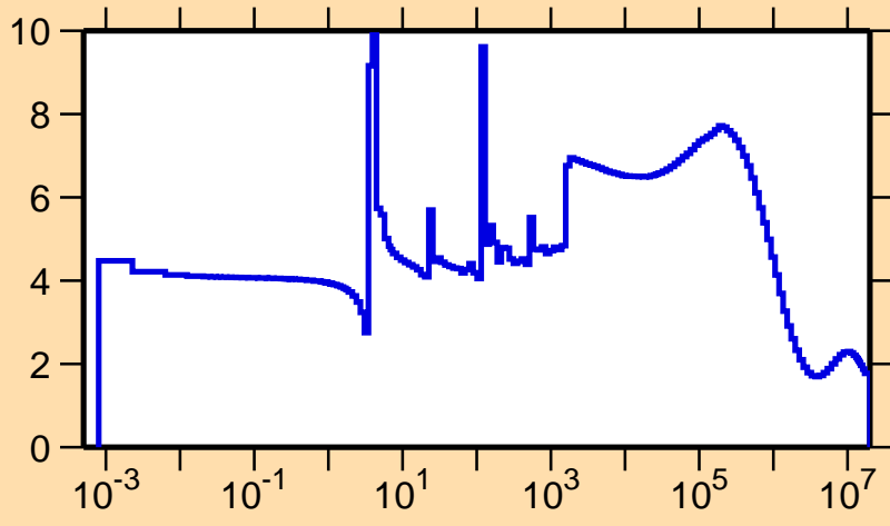
\sigma vs. E for ^{87}\text{Zr}(n,\text{el.})
