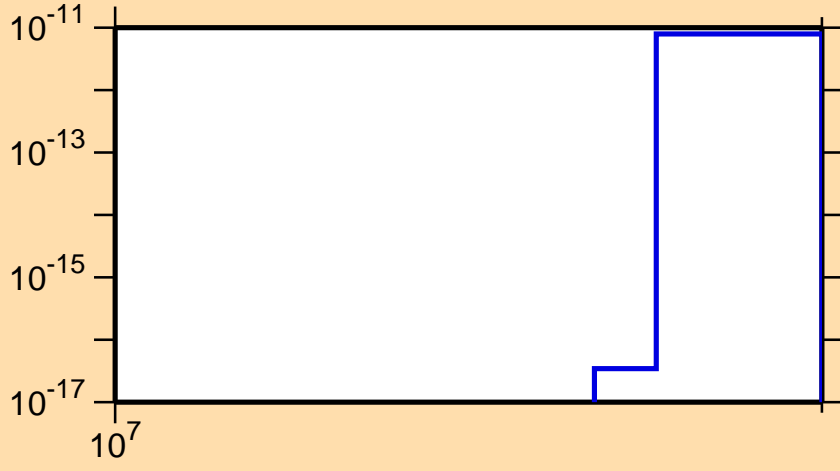
\sigma vs. E for ^{87}\text{Zr} (mt 34)
