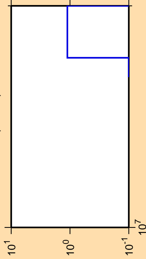
\Delta\sigma/\sigma vs. E for ^{87}\text{Zr} (mt 45)
