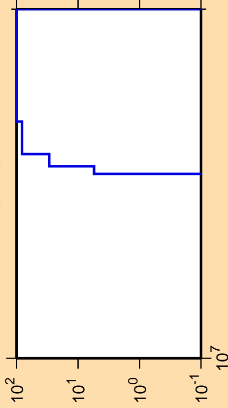
\Delta\sigma/\sigma vs. E for ^{87}\text{Zr}(n,nd)
