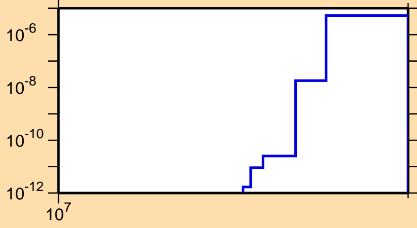
\sigma vs. E for ^{87}\text{Zr}(n,nd)
