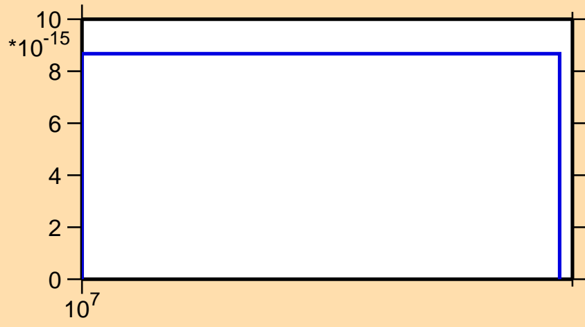
\sigma vs. E for ^{87}\text{Zr} (mt 45)
