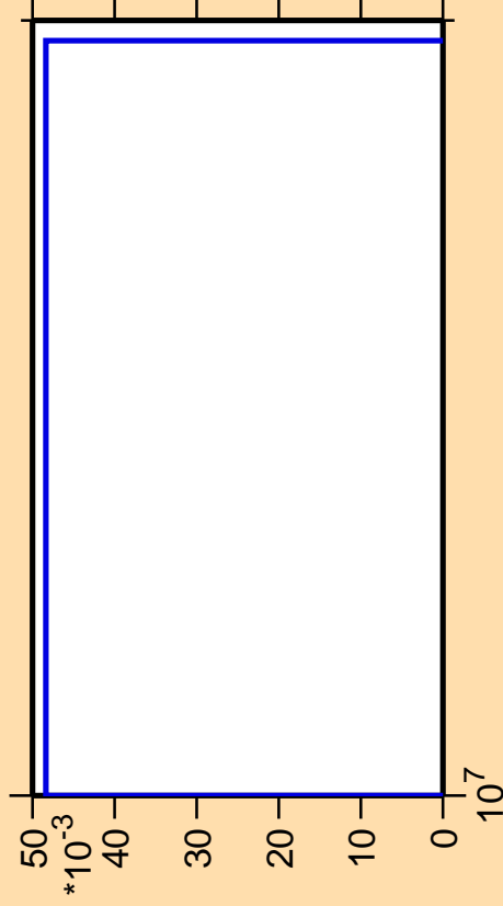
\Delta\sigma/\sigma vs. E for ^{87}\text{Zr} (mt 45)
