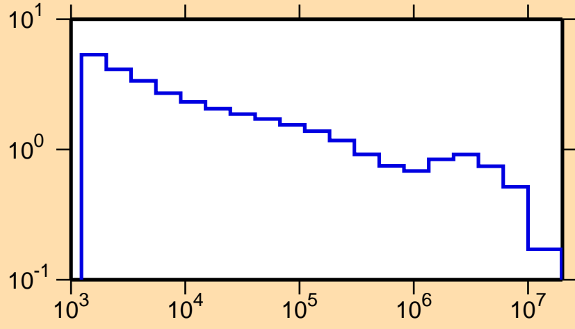
\sigma vs. E for ^{87}\text{Zr}(n,p)
