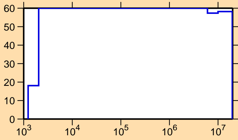
\Delta\sigma/\sigma vs. E for ^{87}\text{Zr}(n,\gamma)
