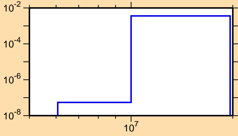
\sigma vs. E for ^{87}\text{Zr}(n,n\alpha)
