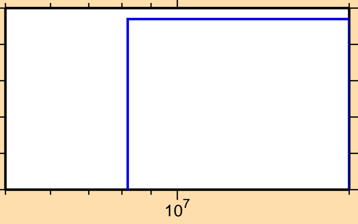
\sigma vs. E for ^{87}\text{Zr}(n,2n)
