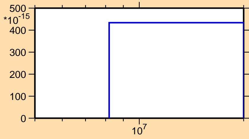
\sigma vs. E for ^{87}\text{Zr}(\text{mt } 34)
