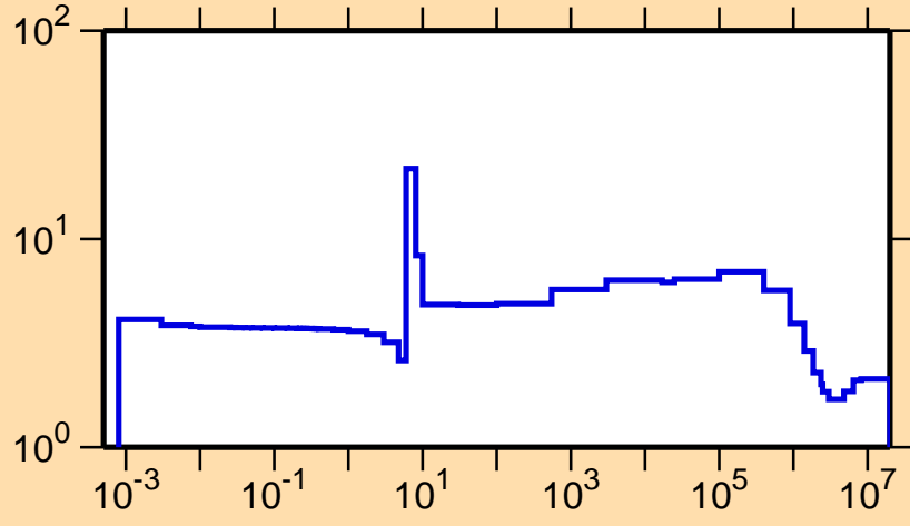
\sigma vs. E for ^{87}\text{Zr}(n,\text{el.})
