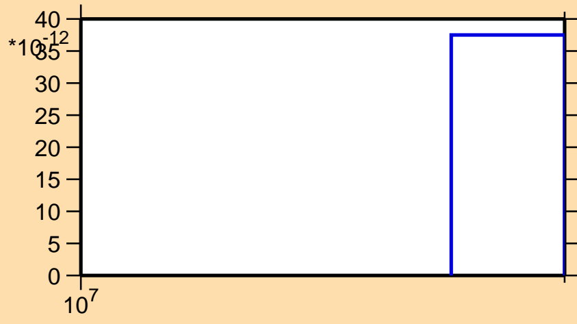
\sigma vs. E for ^{88}\text{Zr}(n,\text{nd})
