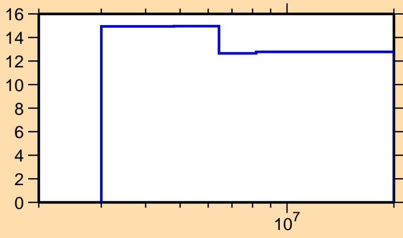
\Delta\sigma/\sigma vs. E for ^{88}\text{Zr}(n,n\text{onel.})
