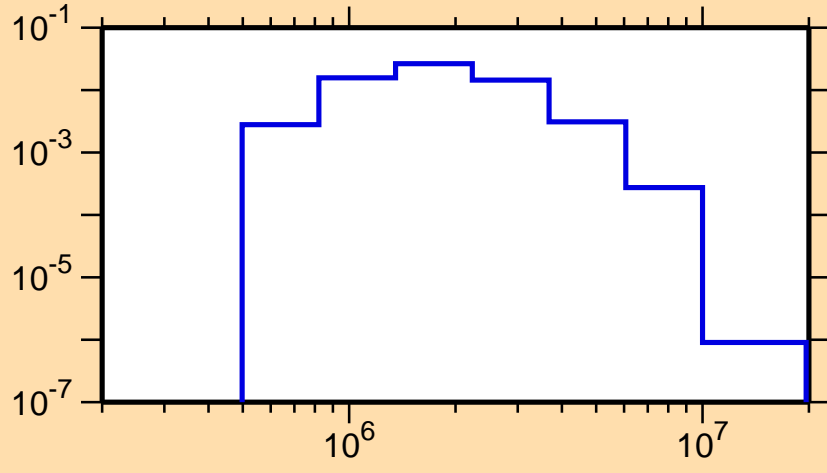
\sigma vs. E for ^{89}\text{Zr}(n,n_1)
