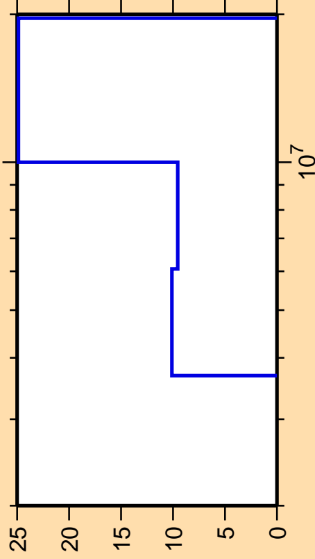
\Delta\sigma/\sigma vs. E for ^{90}\text{Zr}(n,n_{\text{cont}}) .
