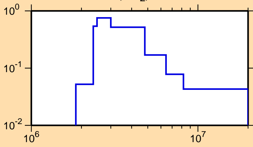
\sigma vs. E for ^{90}\text{Zr}(n,n_2)
