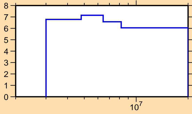
\Delta\sigma/\sigma vs. E for ^{90}\text{Zr}(n,n\text{onel.})
