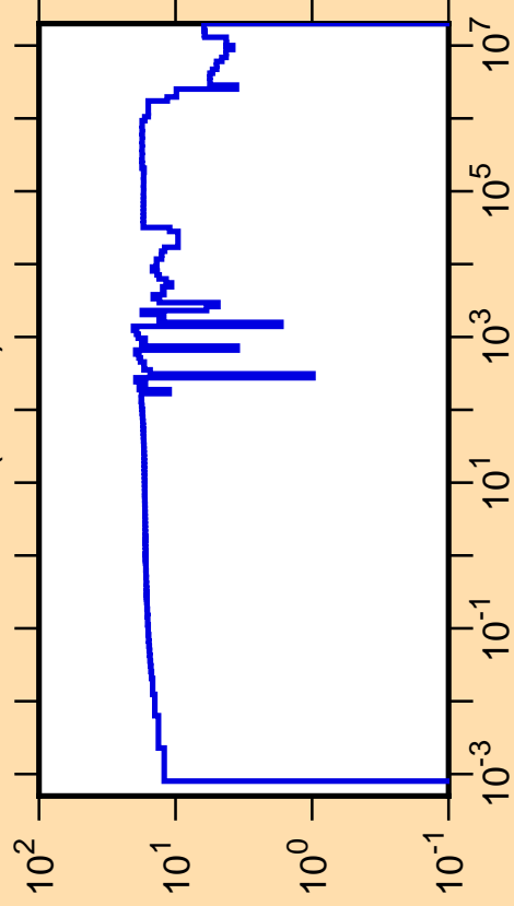
\Delta\sigma/\sigma vs. E for ^{91}\text{Zr}(n,\text{tot.})
