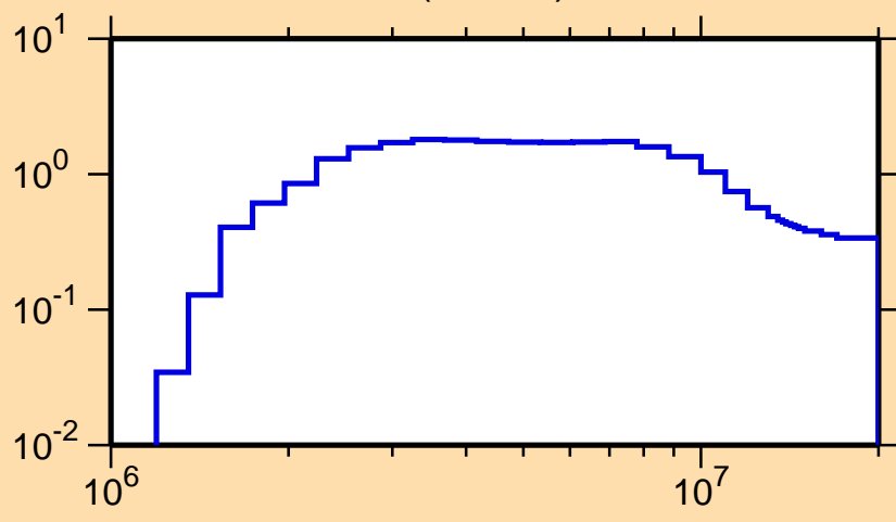
\sigma vs. E for ^{91}\text{Zr}(n,\text{inel.})
