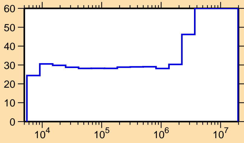
\Delta\sigma/\sigma vs. E for ^{91}\text{Zr}(n,\gamma)
