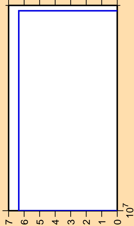
\Delta\sigma/\sigma vs. E for ^{91}\text{Zr}(n,\text{pt})
