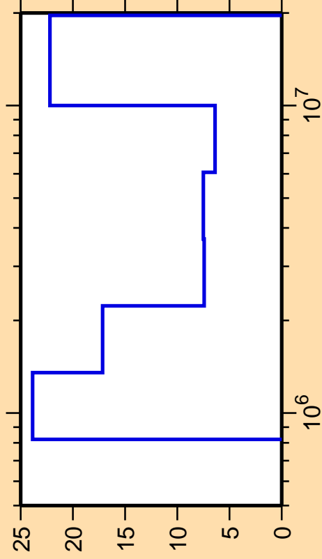
\Delta\sigma/\sigma vs. E for ^{91}\text{Zr}(n,\text{inel.})
