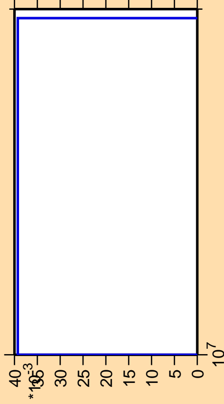
\Delta\sigma/\sigma vs. E for ^{91}\text{Zr}(n,\text{pd})
