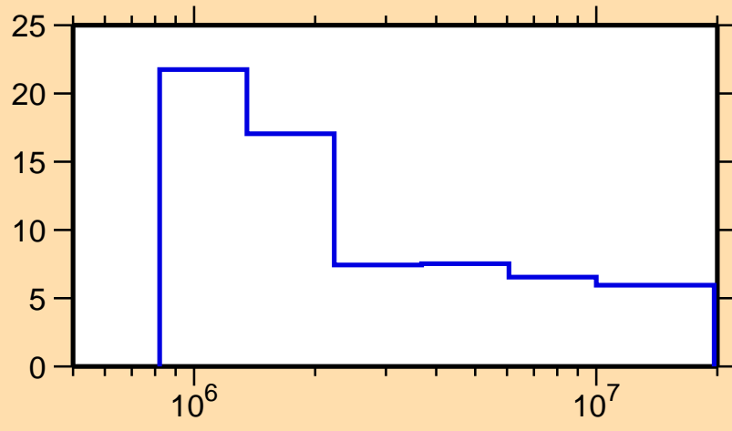
\Delta\sigma/\sigma vs. E for ^{91}\text{Zr}(n,\text{nonel.})
