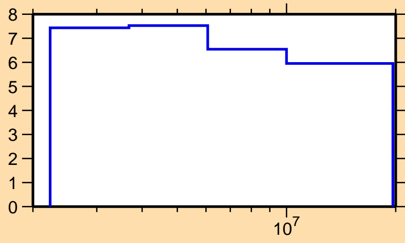
\Delta\sigma/\sigma vs. E for ^{91}\text{Zr}(n,n\text{onel.})
