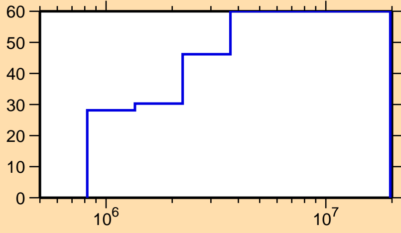
\Delta\sigma/\sigma vs. E for ^{91}\text{Zr}(n,\gamma)
