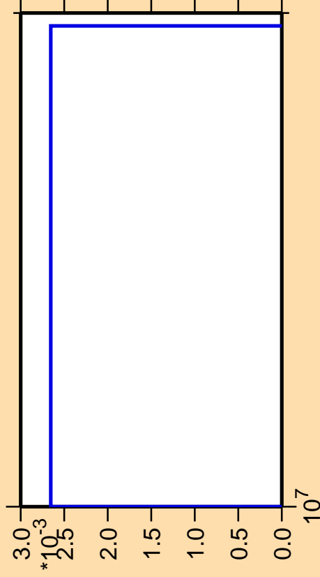
\Delta\sigma/\sigma vs. E for ^{91}\text{Zr} (mt 34)
