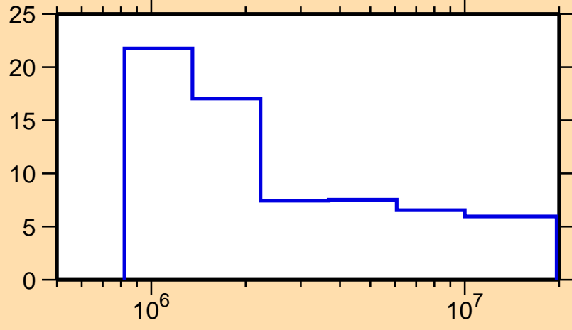
\Delta\sigma/\sigma vs. E for ^{91}\text{Zr}(n,\text{nonel.})
