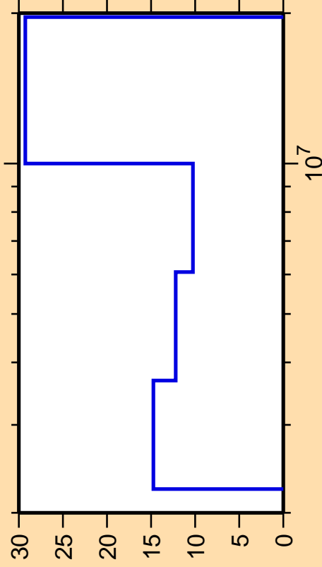
\Delta\sigma/\sigma vs. E for ^{91}\text{Zr}(n,\text{ncont.})
