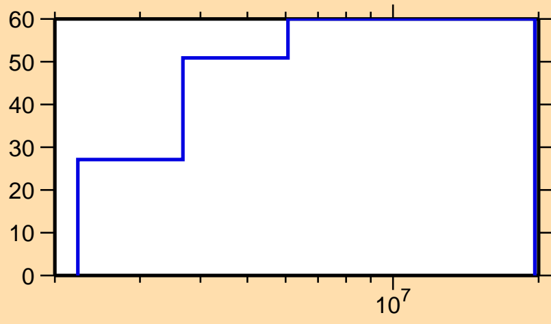
\Delta\sigma/\sigma vs. E for ^{91}\text{Zr}(n,n_1)
