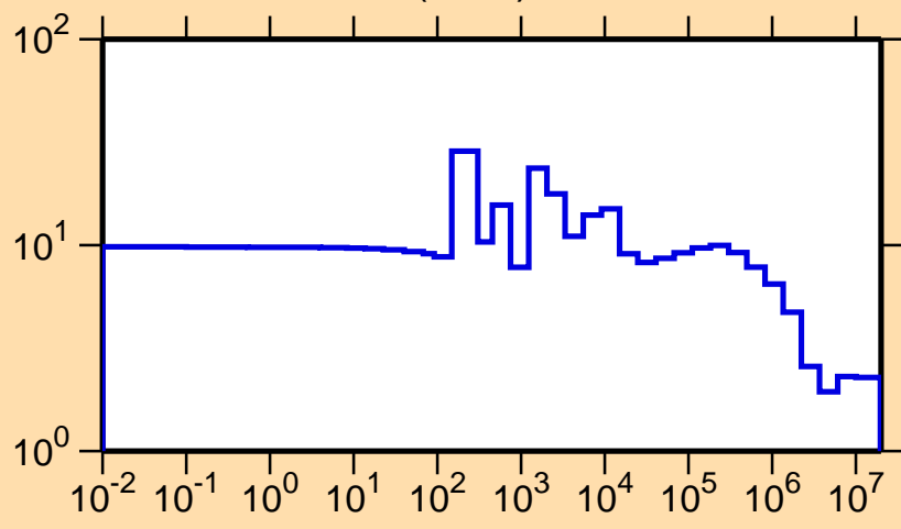
\sigma vs. E for ^{91}\text{Zr}(n,\text{el.})
