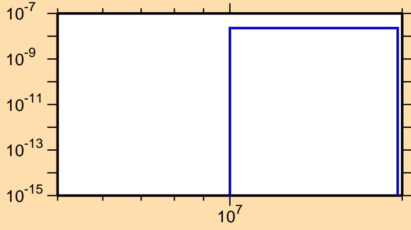
\sigma vs. E for ^{91}\text{Zr}(n,p\alpha)
