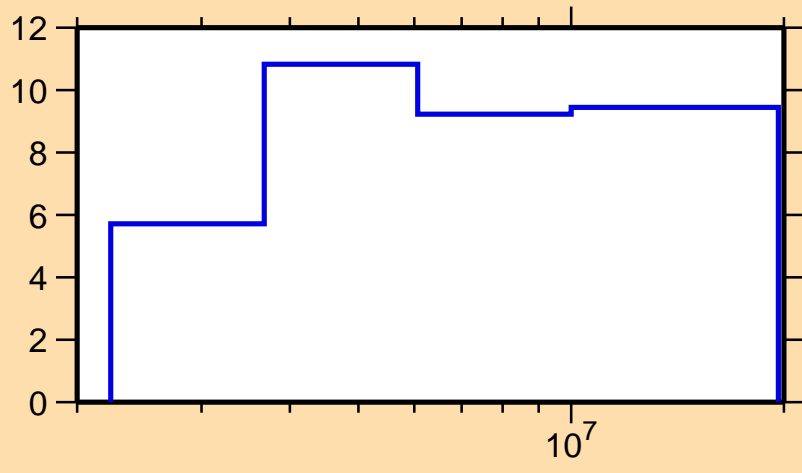
\Delta\sigma/\sigma vs. E for ^{91}\text{Zr}(n,\text{el.})
