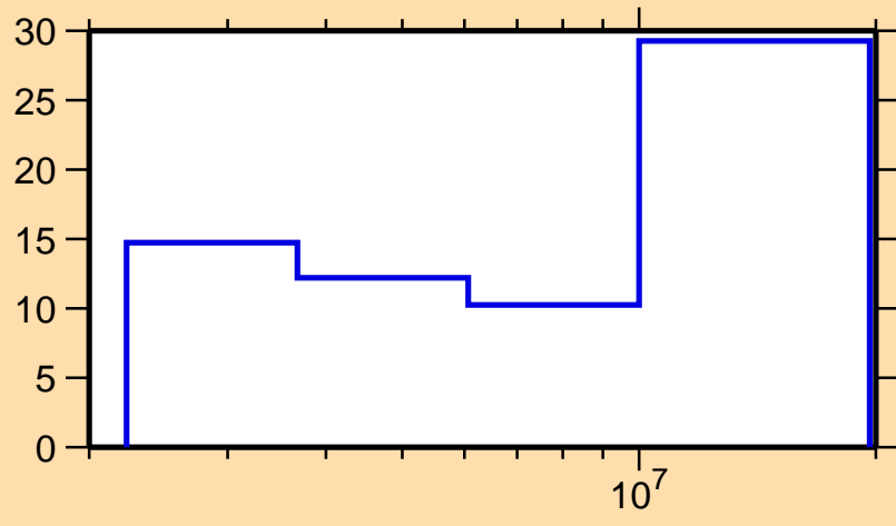
\Delta\sigma/\sigma vs. E for ^{91}\text{Zr}(n,n\text{cont.})
