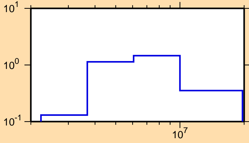
\sigma vs. E for ^{91}\text{Zr}(n,n\text{cont.})
