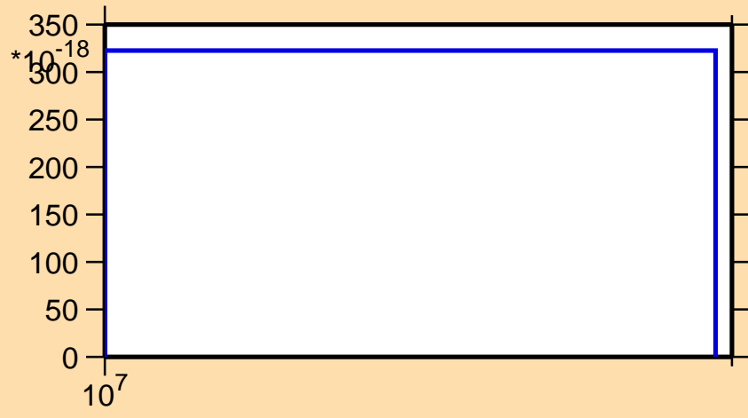
\sigma vs. E for ^{91}\text{Zr} (mt 34)
