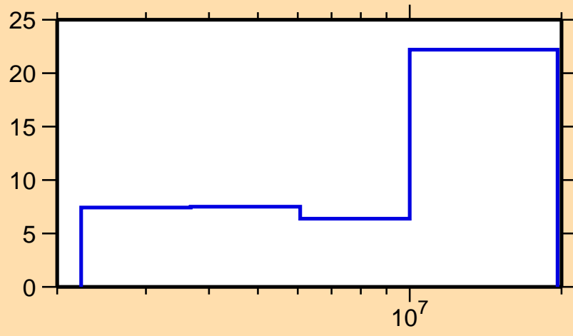
\Delta\sigma/\sigma vs. E for ^{91}\text{Zr}(n,\text{inel.})
