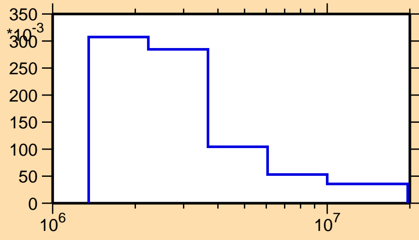
\sigma vs. E for ^{91}\text{Zr}(n,n_2)
