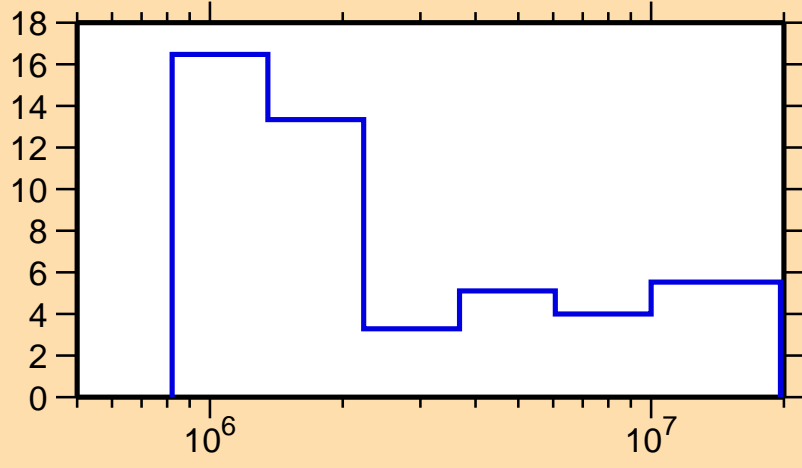
\Delta\sigma/\sigma vs. E for ^{91}\text{Zr}(n,\text{tot.})
