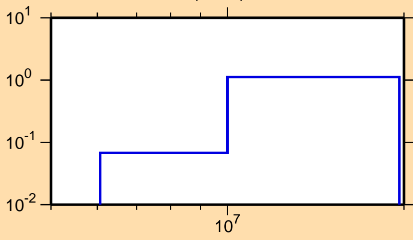
\sigma vs. E for ^{91}\text{Zr}(n,2n)
