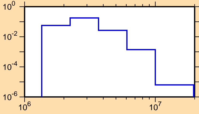
\sigma vs. E for ^{91}\text{Zr}(n,n_3)
