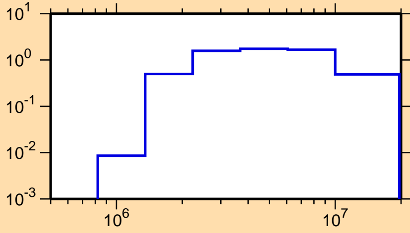
\sigma vs. E for ^{91}\text{Zr}(n,\text{inel.})
