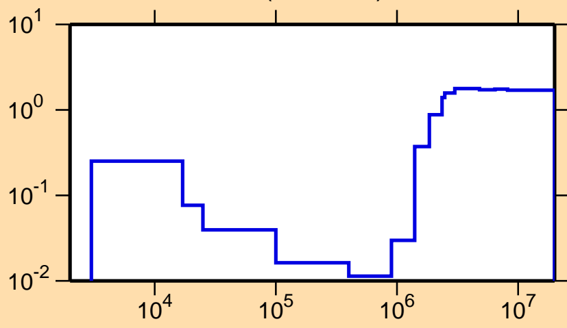
\sigma vs. E for ^{91}\text{Zr}(n,\text{nonel.})
