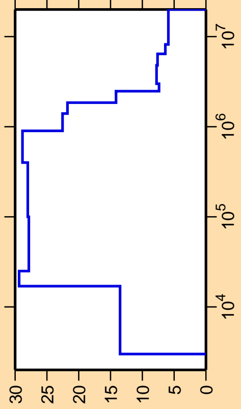
\Delta\sigma/\sigma vs. E for ^{91}\text{Zr}(n,\text{nonel.})
