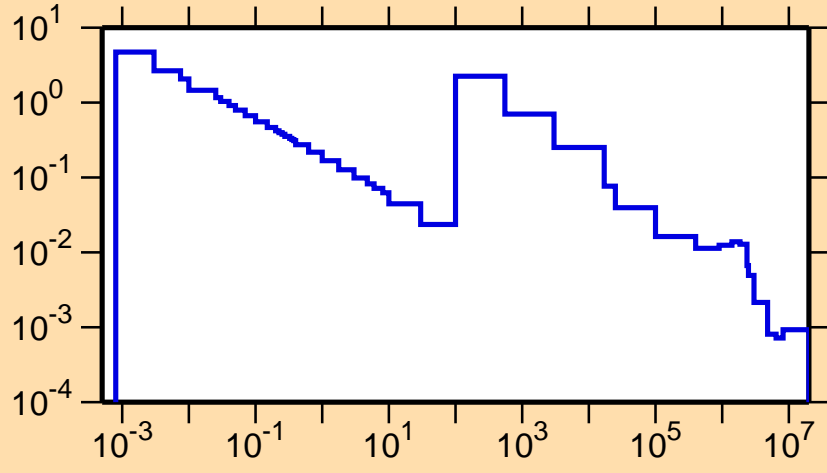
\sigma vs. E for ^{91}\text{Zr}(n,\gamma)
