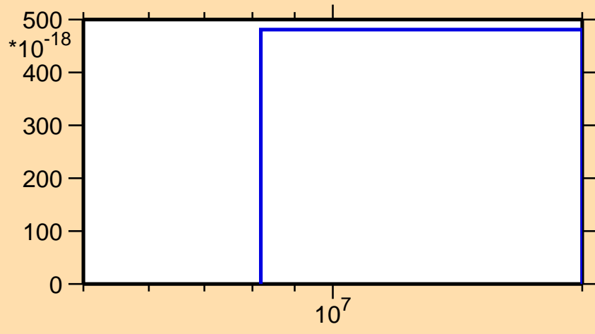
\sigma vs. E for ^{91}\text{Zr}(\text{mt } 34)
