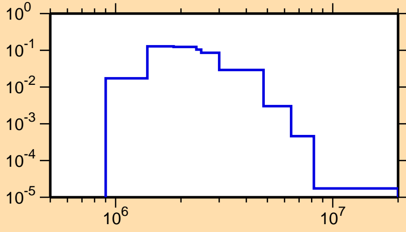
\sigma vs. E for ^{91}\text{Zr}(n,n_1)
