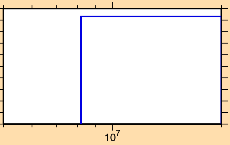
\sigma vs. E for ^{91}\text{Zr}(n,p\alpha)
