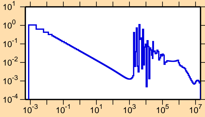
\sigma vs. E for ^{92}\text{Zr}(n,\gamma)
