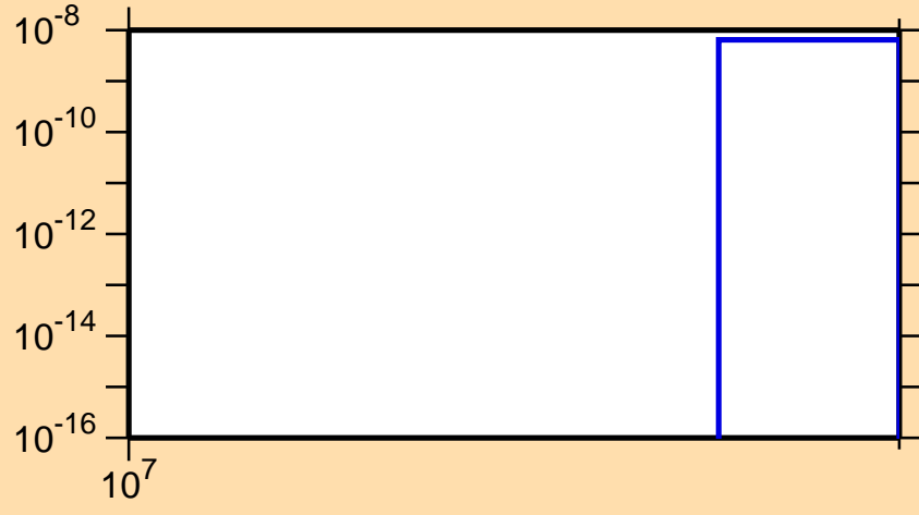
\sigma vs. E for ^{92}\text{Zr}(n,nt)
