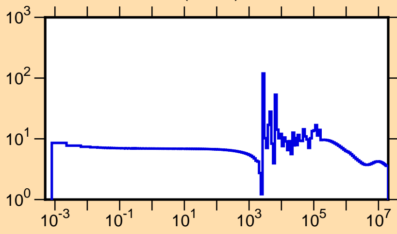
\sigma vs. E for ^{92}\text{Zr}(n,\text{tot.})
