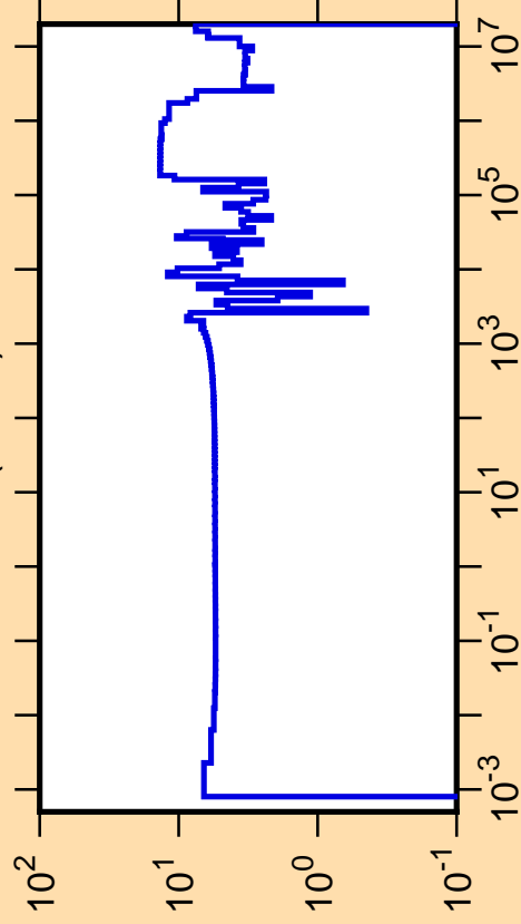
\Delta\sigma/\sigma vs. E for ^{92}\text{Zr}(n,\text{tot.})
