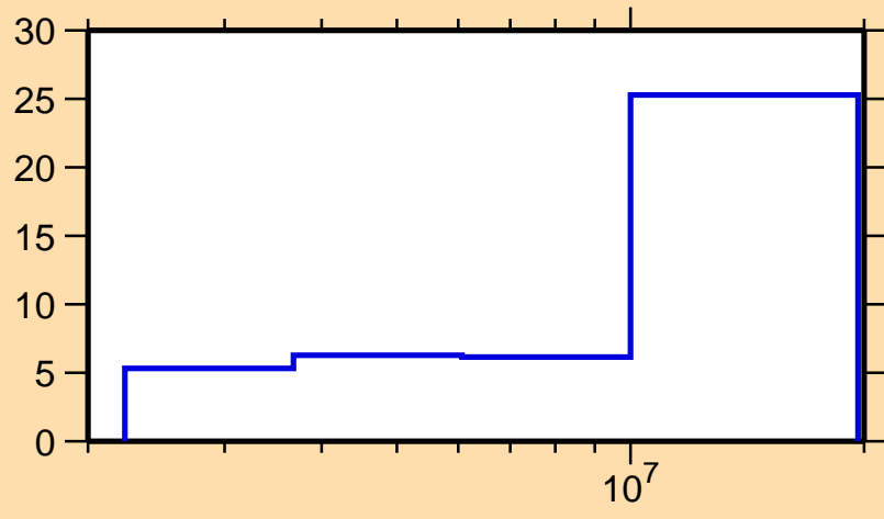
\Delta\sigma/\sigma vs. E for ^{92}\text{Zr}(n,inel.)
