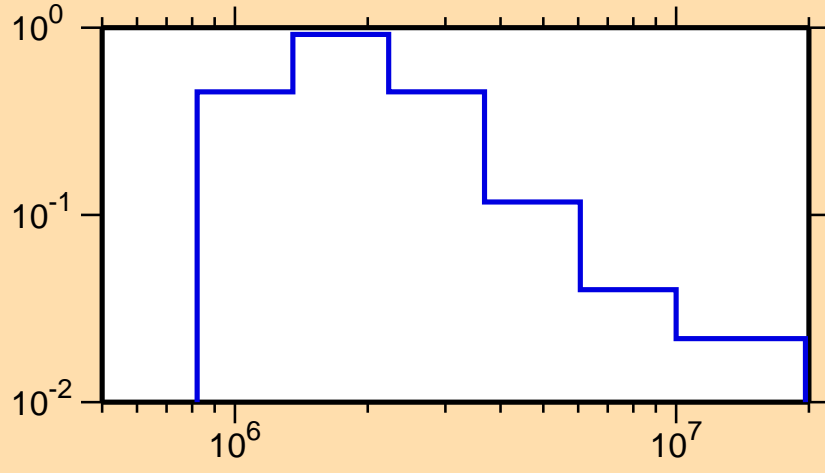
\sigma vs. E for ^{92}\text{Zr}(n,n_1)
