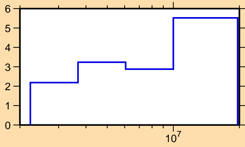
\Delta\sigma/\sigma vs. E for ^{92}\text{Zr}(n,tot.)
