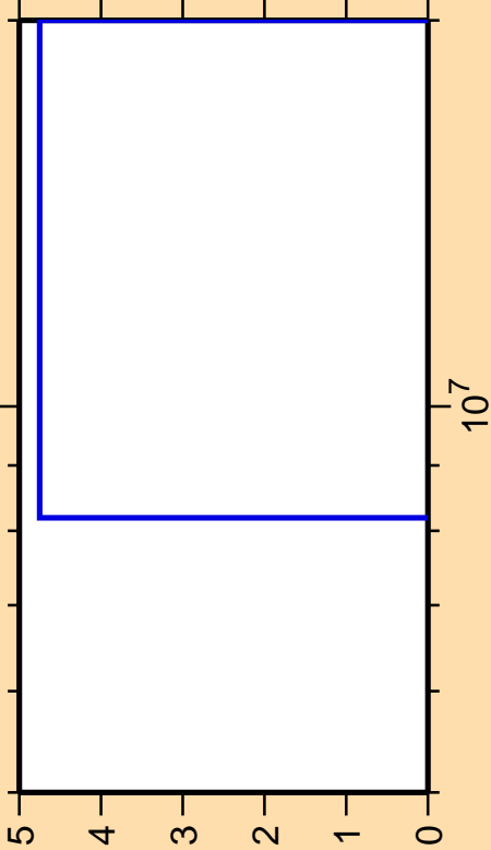
\Delta\sigma/\sigma vs. E for ^{92}\text{Zr}(n,2n\alpha)
