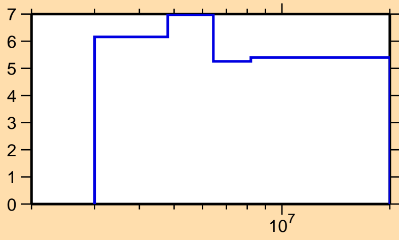
\Delta\sigma/\sigma vs. E for ^{92}\text{Zr}(n,n\text{onel.})
