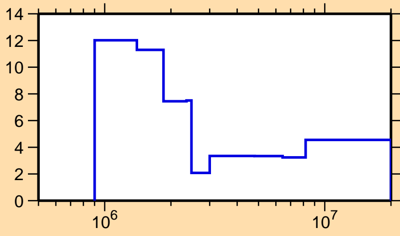
\Delta\sigma/\sigma vs. E for ^{92}\text{Zr}(n,\text{tot.})
