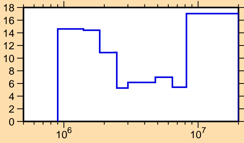
\Delta\sigma/\sigma vs. E for ^{92}\text{Zr}(n,\text{inel.})
