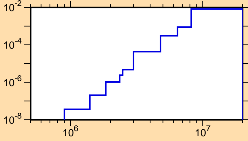
\sigma vs. E for ^{92}\text{Zr}(n,\alpha)
