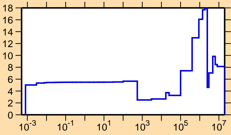
\Delta\sigma/\sigma vs. E for ^{92}\text{Zr}(n,\text{el.})
