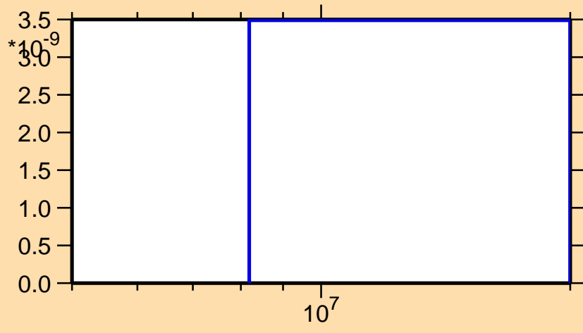
\sigma vs. E for ^{92}\text{Zr}(n,\text{nd})
