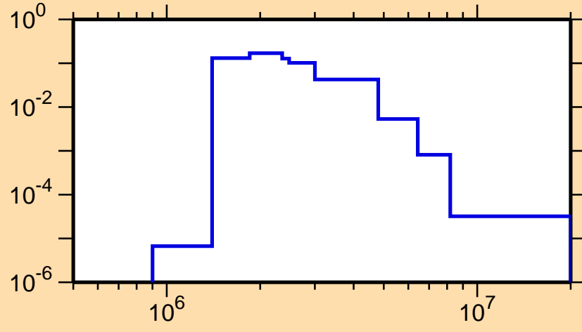
\sigma vs. E for ^{92}\text{Zr}(n,n_2)
