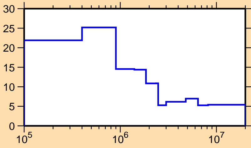
\Delta\sigma/\sigma vs. E for ^{92}\text{Zr}(n,\text{nonel.})
