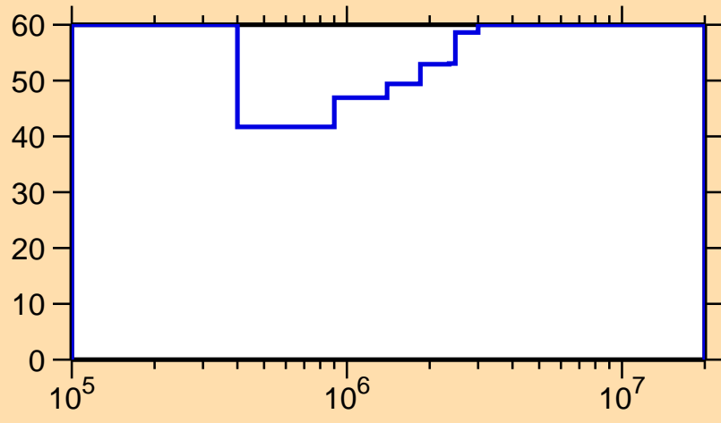
\Delta\sigma/\sigma vs. E for ^{92}\text{Zr}(n,\gamma)
