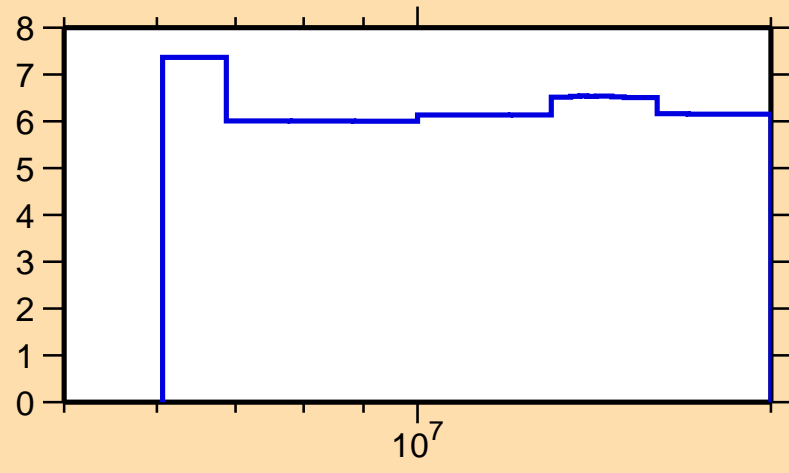
\Delta\sigma/\sigma vs. E for ^{93}\text{Zr}(n,\text{nonel.})
