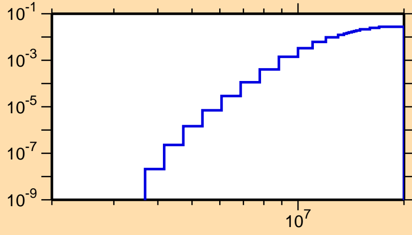
\sigma vs. E for ^{93}\text{Zr}(n,p)
