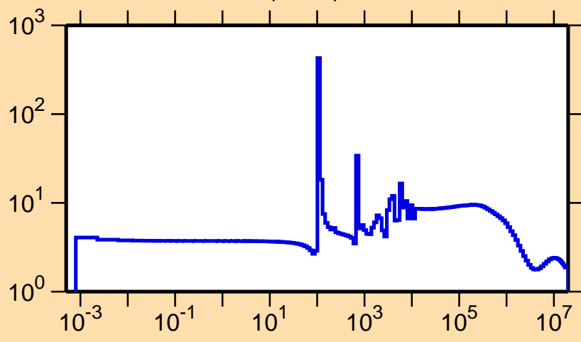
\sigma vs. E for ^{93}\text{Zr}(n,\text{el.})
