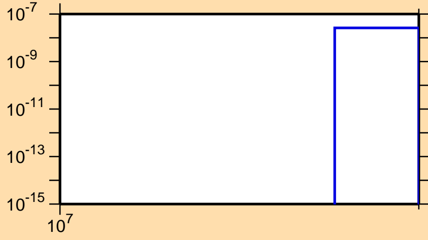
\sigma vs. E for ^{93}\text{Zr}(n,\text{nt})
