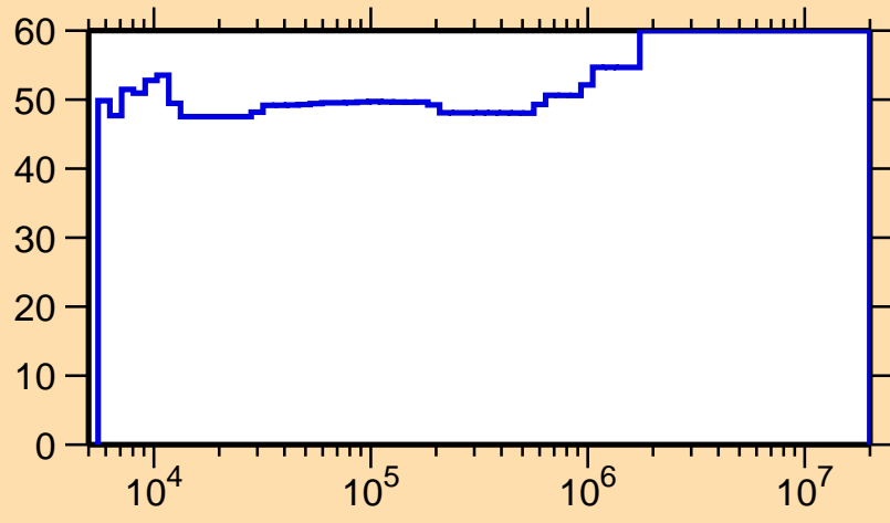
\Delta\sigma/\sigma vs. E for ^{93}\text{Zr}(n,\gamma)
