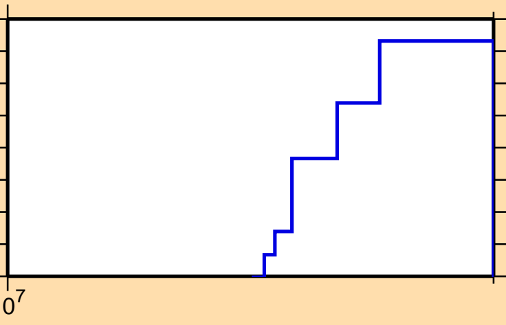
\sigma vs. E for ^{93}\text{Zr}(n,\text{He}3)
