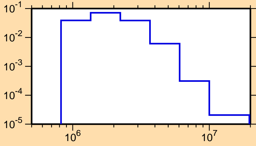
\sigma vs. E for ^{93}\text{Zr}(n,n_2)
