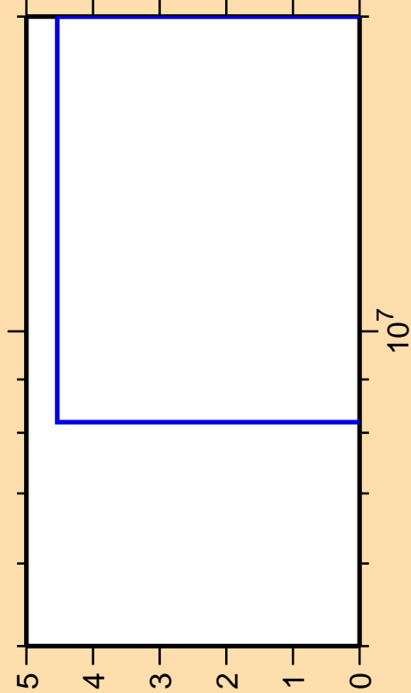
\Delta\sigma/\sigma vs. E for ^{93}\text{Zr}(n,p\alpha)
