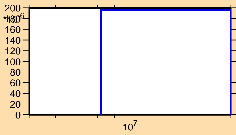
\sigma vs. E for ^{93}\text{Zr}(n,t)
