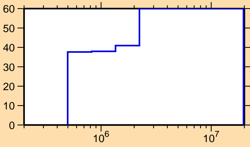
\Delta\sigma/\sigma vs. E for ^{95}\text{Zr}(n,\gamma)
