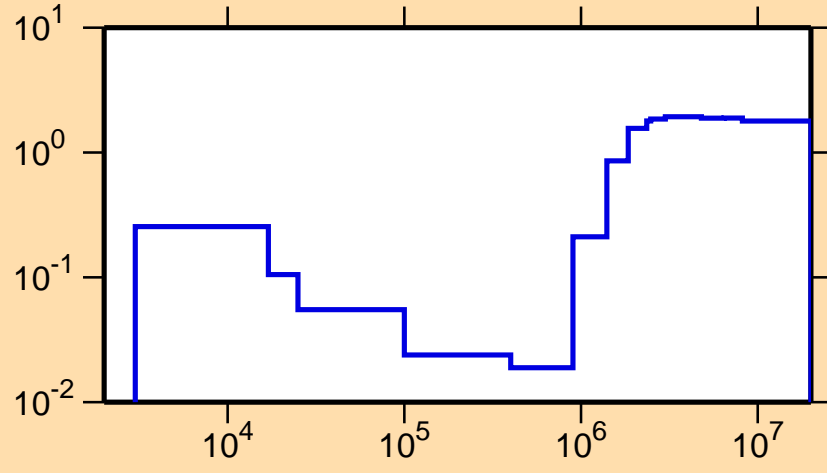
\sigma vs. E for ^{95}\text{Zr}(n,\text{nonel.})
