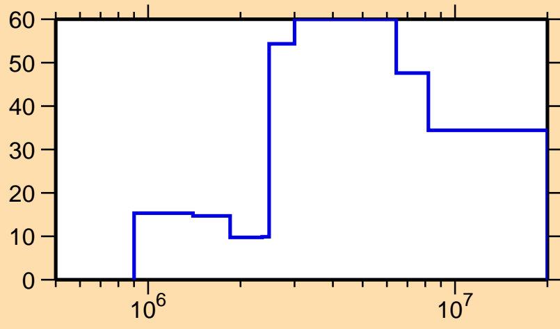
\Delta\sigma/\sigma vs. E for ^{95}\text{Zr}(n,n_1)
