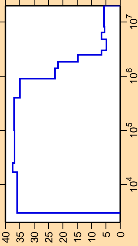
\Delta\sigma/\sigma vs. E for ^{95}\text{Zr}(n,\text{nonel.})
