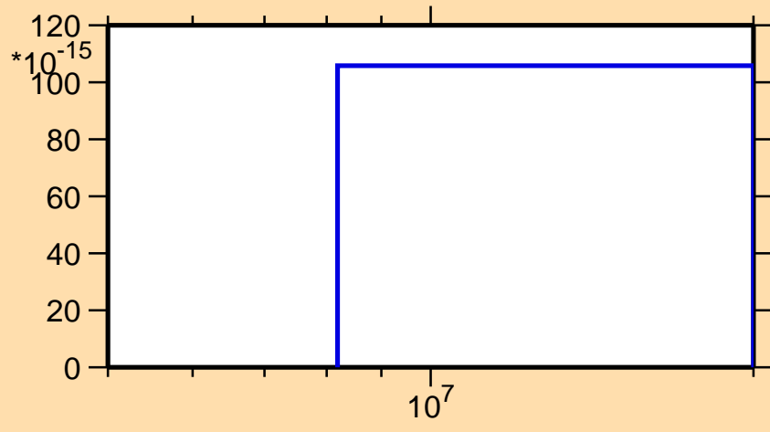
\sigma vs. E for ^{95}\text{Zr}(n,\text{He}3)
