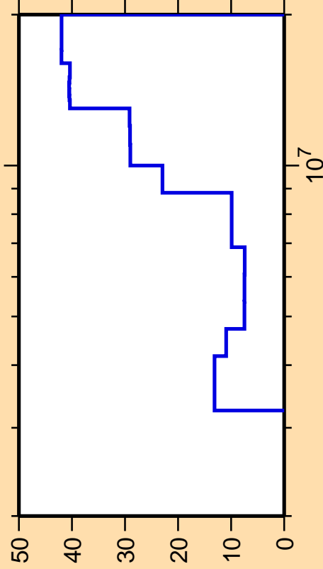
\Delta\sigma/\sigma vs. E for ^{96}\text{Zr}(n,\text{ncont.})
