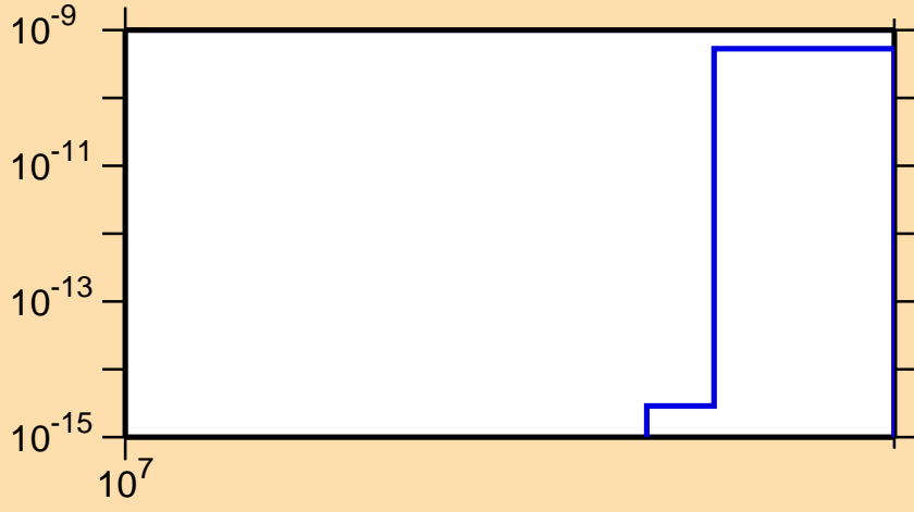
\sigma vs. E for ^{96}\text{Zr}(n,nt)
