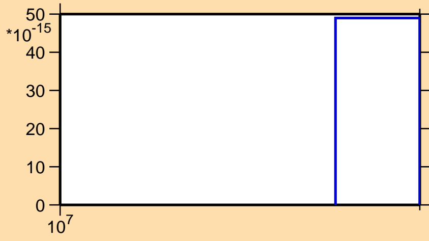
\sigma vs. E for ^{96}\text{Zr}(n,2np)
