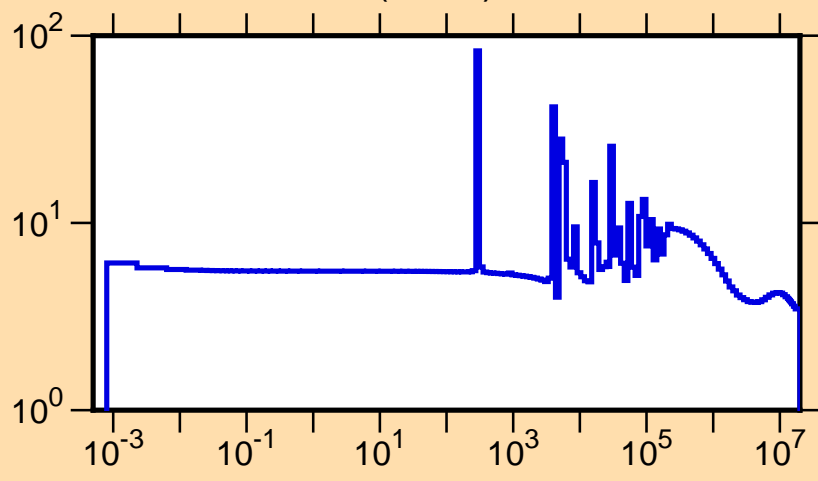
\sigma vs. E for ^{96}\text{Zr}(n,\text{tot.})
