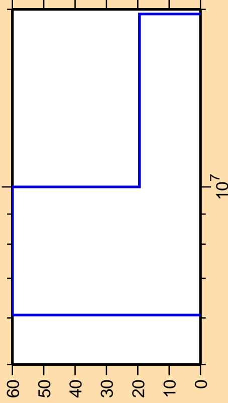
\Delta\sigma/\sigma vs. E for ^{96}\text{Zr}(n,\alpha)
