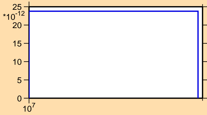
\sigma vs. E for ^{96}\text{Zr}(n,nd)
