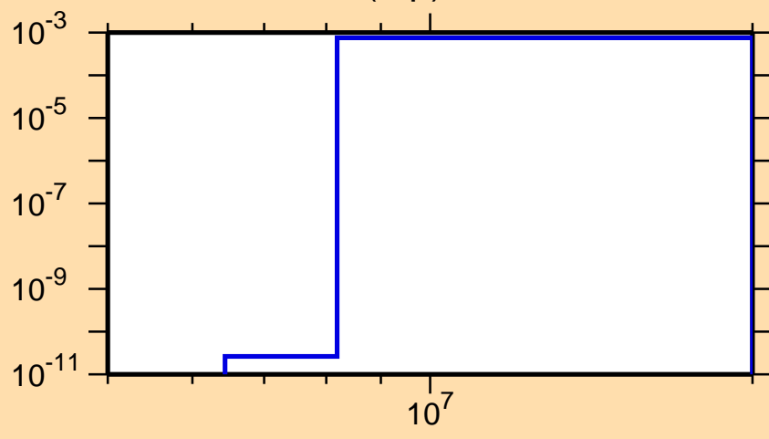
\sigma vs. E for ^{96}\text{Zr}(n,p)
