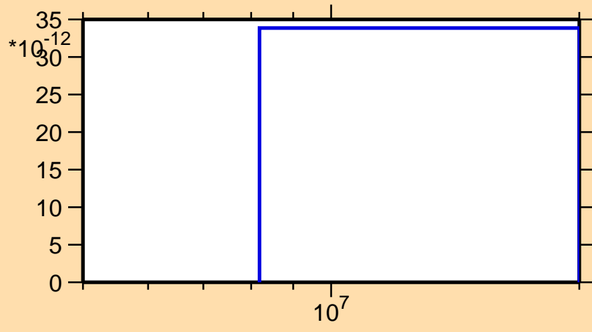
\sigma vs. E for ^{96}\text{Zr}(n,\text{nd})
