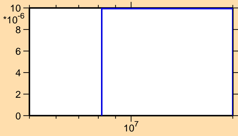
\sigma vs. E for ^{96}\text{Zr}(n,np)
