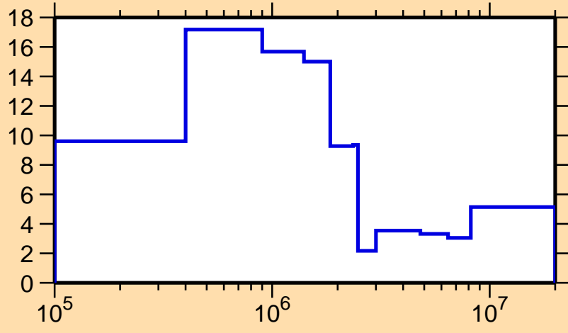
\Delta\sigma/\sigma vs. E for ^{96}\text{Zr}(n,\text{tot.})
