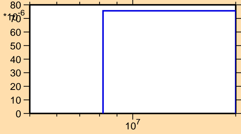
\sigma vs. E for ^{96}\text{Zr}(n,d)
