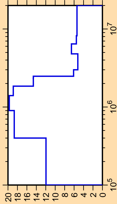
\Delta\sigma/\sigma vs. E for ^{96}\text{Zr}(n,\text{nonel.})
