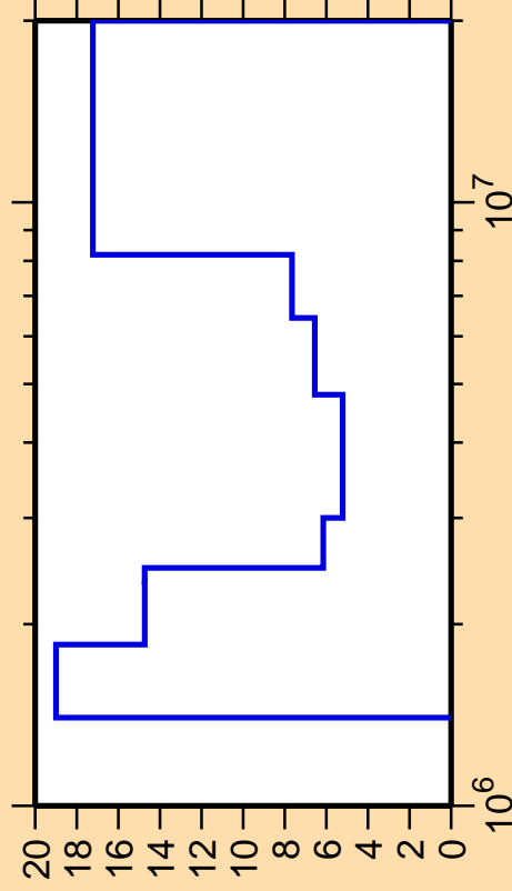
\Delta\sigma/\sigma vs. E for ^{96}\text{Zr}(n,\text{inel.})
