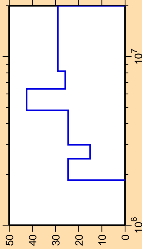
\Delta\sigma/\sigma vs. E for ^{96}\text{Zr}(n,n_4)
