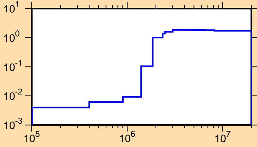
\sigma vs. E for ^{96}\text{Zr}(n,\text{nonel.})
