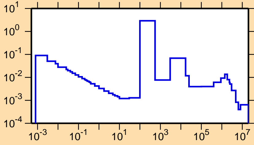
\sigma vs. E for ^{96}\text{Zr}(n,\gamma)
