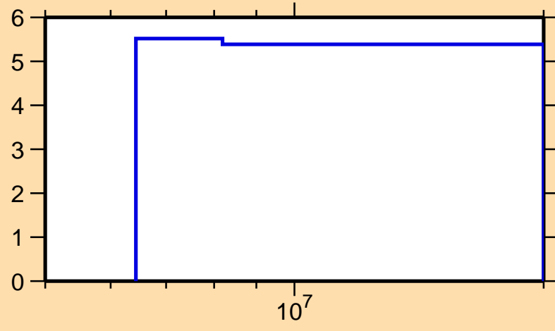
\Delta\sigma/\sigma vs. E for ^{96}\text{Zr}(n,\text{nonel.})
