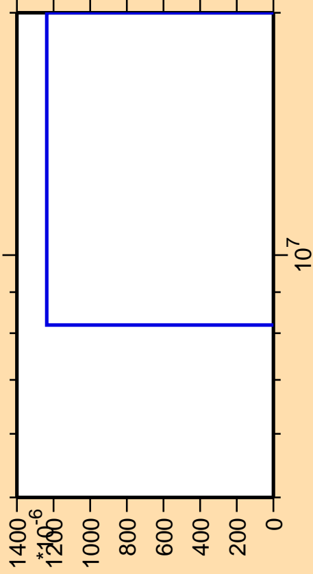
\Delta\sigma/\sigma vs. E for ^{96}\text{Zr}(n,2np)
