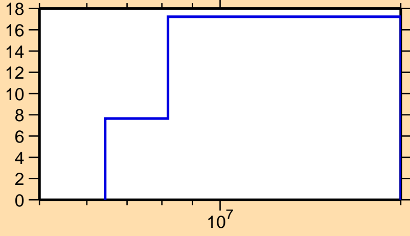
\Delta\sigma/\sigma vs. E for ^{96}\text{Zr}(n,\text{inel.})
