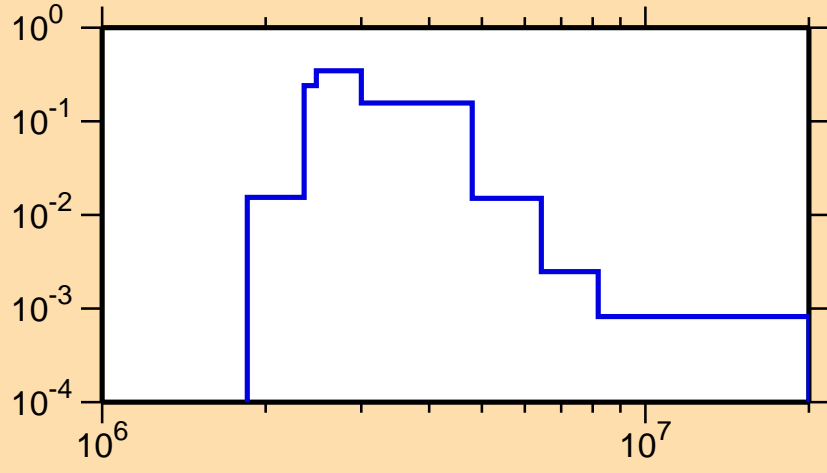
\sigma vs. E for ^{96}\text{Zr}(n,n_4)
