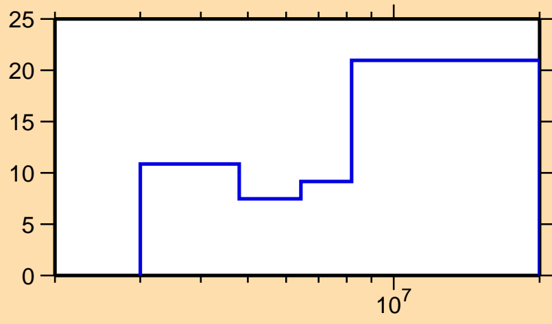
\Delta\sigma/\sigma vs. E for ^{96}\text{Zr}(n,n\text{cont.})
