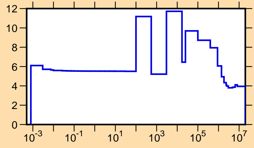
\sigma vs. E for ^{96}\text{Zr}(n,\text{tot.})
