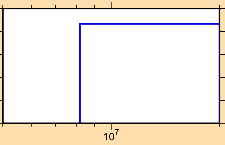
\sigma vs. E for ^{96}\text{Zr}(n,nt)
