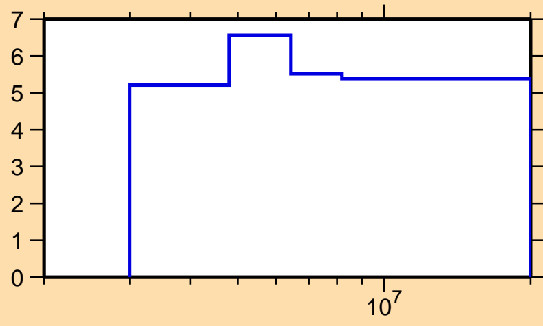
\Delta\sigma/\sigma vs. E for ^{96}\text{Zr}(n,n\text{onel.})
