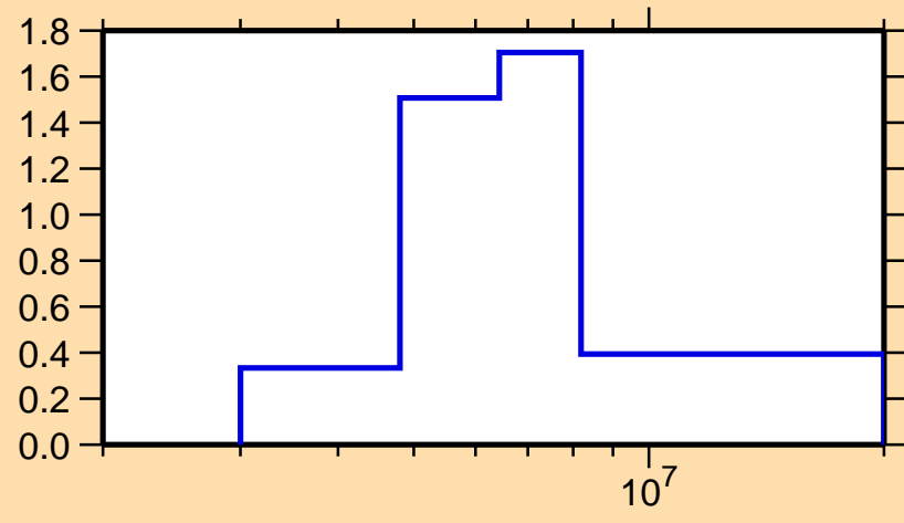
\sigma vs. E for ^{96}\text{Zr}(n,n\text{cont.})
