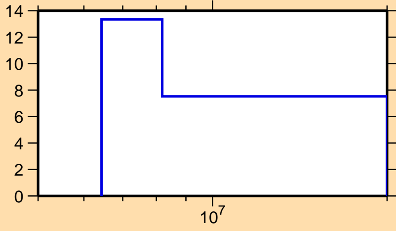
\Delta\sigma/\sigma vs. E for ^{96}\text{Zr}(n,2n)
