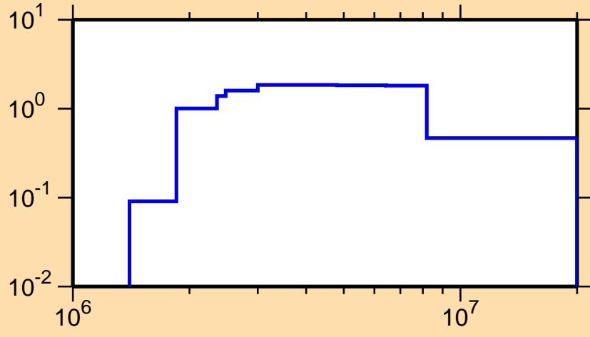
\sigma vs. E for ^{96}\text{Zr}(n,\text{inel.})
