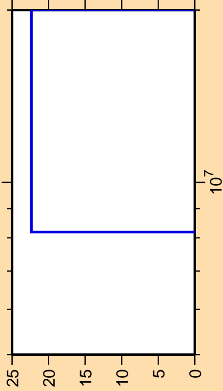
\Delta\sigma/\sigma vs. E for ^{96}\text{Zr}(n,nt)
