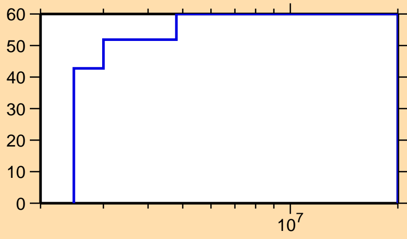
\Delta\sigma/\sigma vs. E for ^{96}\text{Zr}(n,\gamma)
