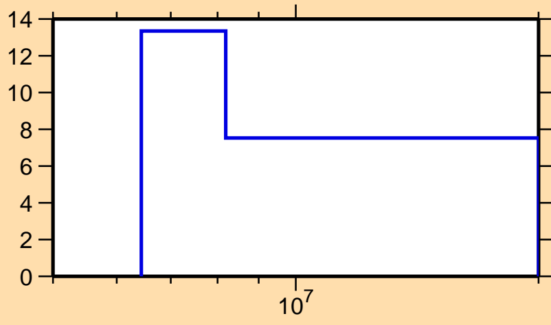
\Delta\sigma/\sigma vs. E for ^{96}\text{Zr}(n,2n)
