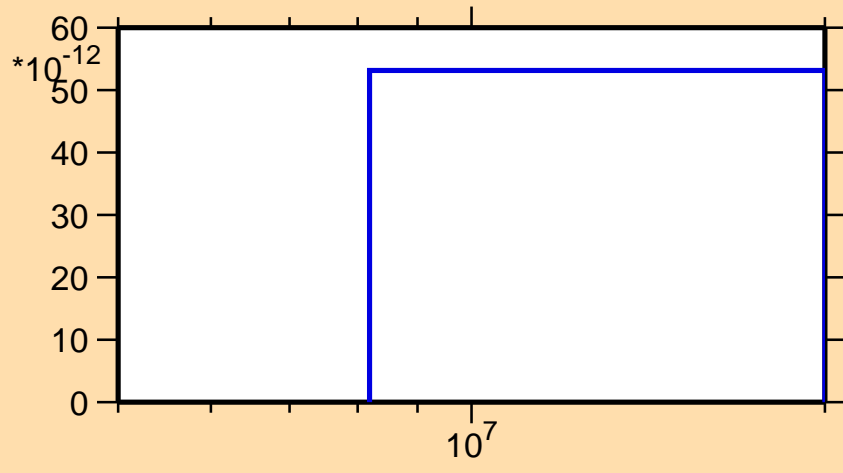
\sigma vs. E for ^{96}\text{Zr}(n,2n\alpha)
