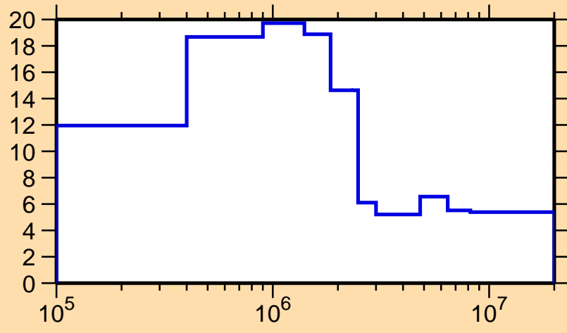
\Delta\sigma/\sigma vs. E for ^{96}\text{Zr}(n,\text{nonel.})
