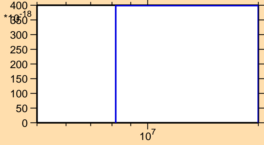
\sigma vs. E for ^{96}\text{Zr}(n,2np)
