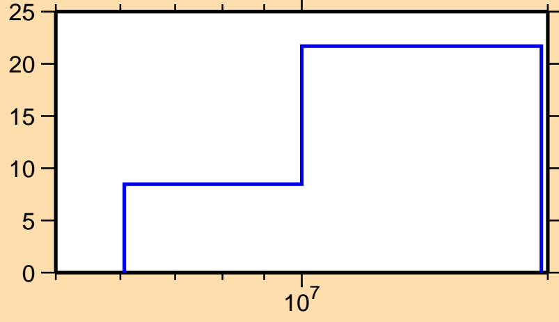
\Delta\sigma/\sigma vs. E for ^{98}\text{Zr}(n,\text{el.})
