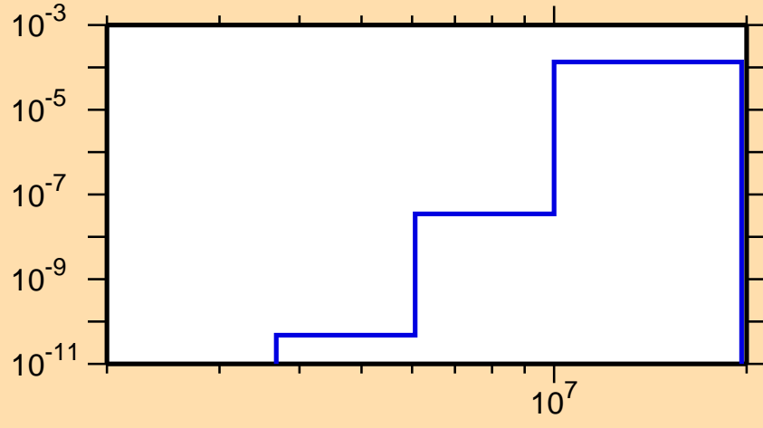
\sigma vs. E for ^{98}\text{Zr}(n,\alpha)
