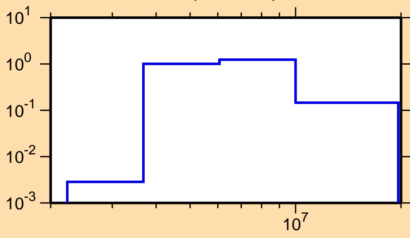
\sigma vs. E for ^{98}\text{Zr}(n,n\text{cont.})
