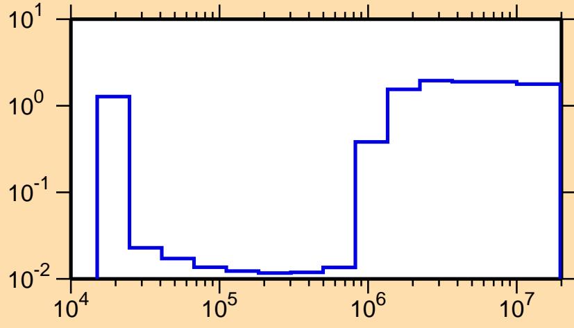
\sigma vs. E for ^{98}\text{Zr}(n,\text{nonel.})
