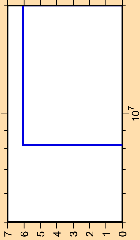
\Delta\sigma/\sigma vs. E for ^{99}\text{Zr}(n,3n)
