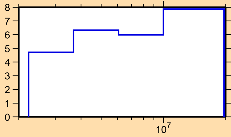
\Delta\sigma/\sigma vs. E for ^{100}\text{Zr}(n,nonel.)
