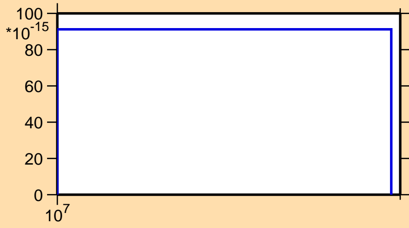
\sigma vs. E for ^{100}\text{Zr}(n,\text{nd})
